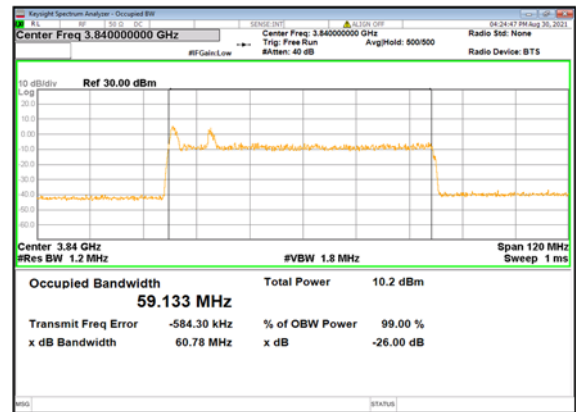
DC_13A_n77 (60M)_DFT-s-OFDM_ QPSK_Outer_Full_Mid_CH
