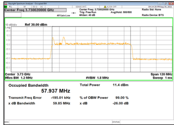
DC_13A_n77 (60M)_DFT-s-OFDM_ QPSK_Outer_Full_Low_CH
