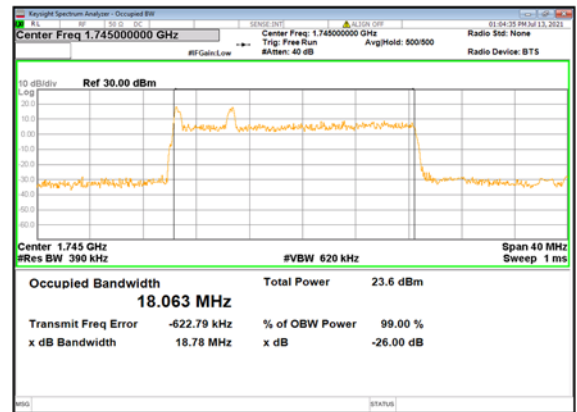
n66(20M)_DFT-s-OFDM_ 64QAM_Outer_Full_Mid_CH
