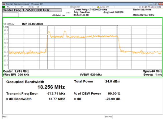
n66(20M)_DFT-s-OFDM_ 16QAM_Outer_Full_Mid_CH
