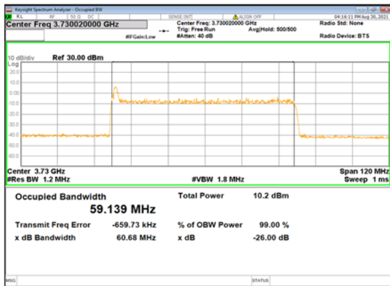
DC_13A_n77 (60M)_DFT-s-OFDM_ 16QAM_Outer_Full_Low_CH
