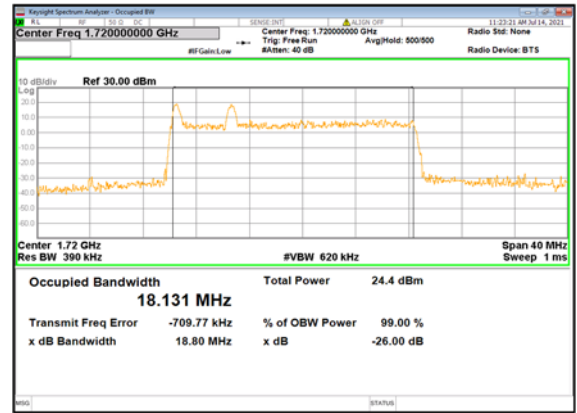
n66(20M)_DFT-s-OFDM_ 64QAM_Outer_Full_Low_CH
