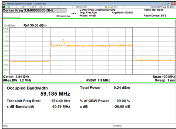
DC_13A_n77 (60M)_DFT-s-OFDM_ 16QAM_Outer_Full_Mid_CH
