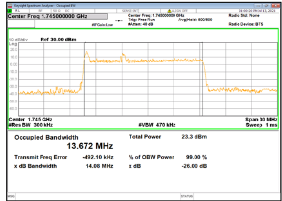
n66(15M)_CP-OFDM_ QPSK_Outer_Full_Mid_CH
