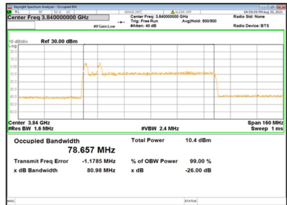
DC_13A_n77 (80M)_DFT-s-OFDM_ 64QAM_Outer_Full_Mid_CH
