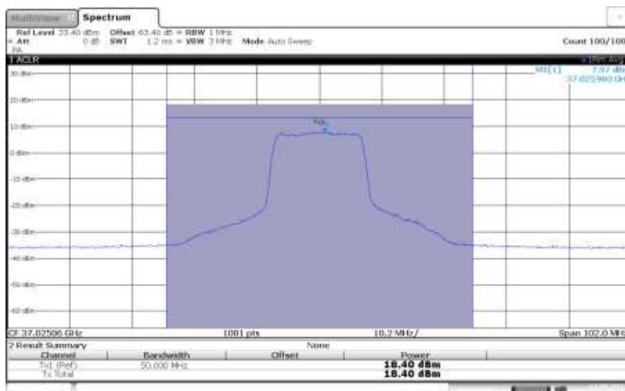
n260, Module1, 50MHz Bandwidth, 10 RB, LOW CHANNEL, QPSK
