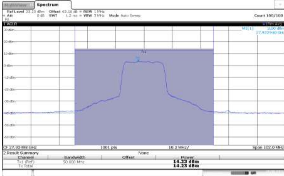
n261, Module1, 50MHz Bandwidth, 10RB, MID CHANNEL, QPSK
