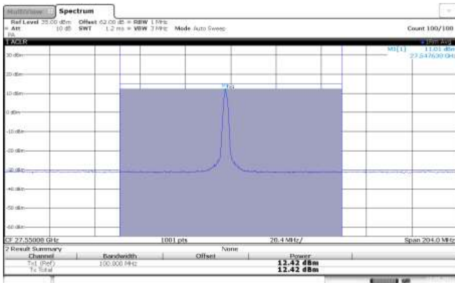
n261, Module1, 100MHz Bandwidth, 1 RB, LOW CHANNEL, QPSK
