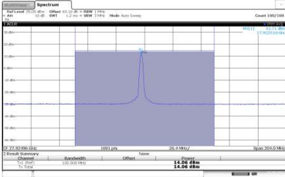
n261, Module1, 100MHz Bandwidth, 1RB, MID CHANNEL, QPSK
