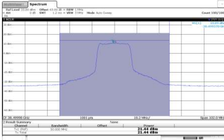
n260, Module1, 50MHz Bandwidth, 10RB, MID CHANNEL, QPSK
