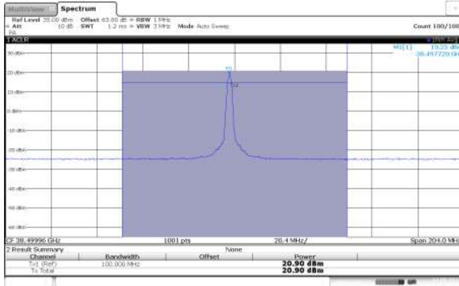
n260, Module1, 100MHz Bandwidth, 1RB, MID CHANNEL, QPSK
