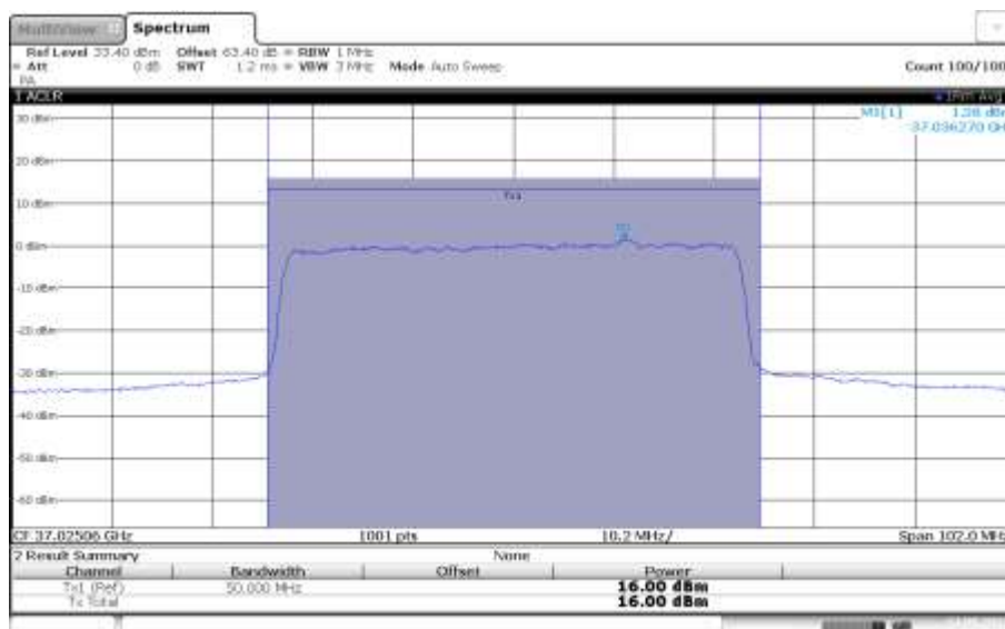
n260, Module1, 50MHz Bandwidth, 100% RB, LOW CHANNEL, QPSK
