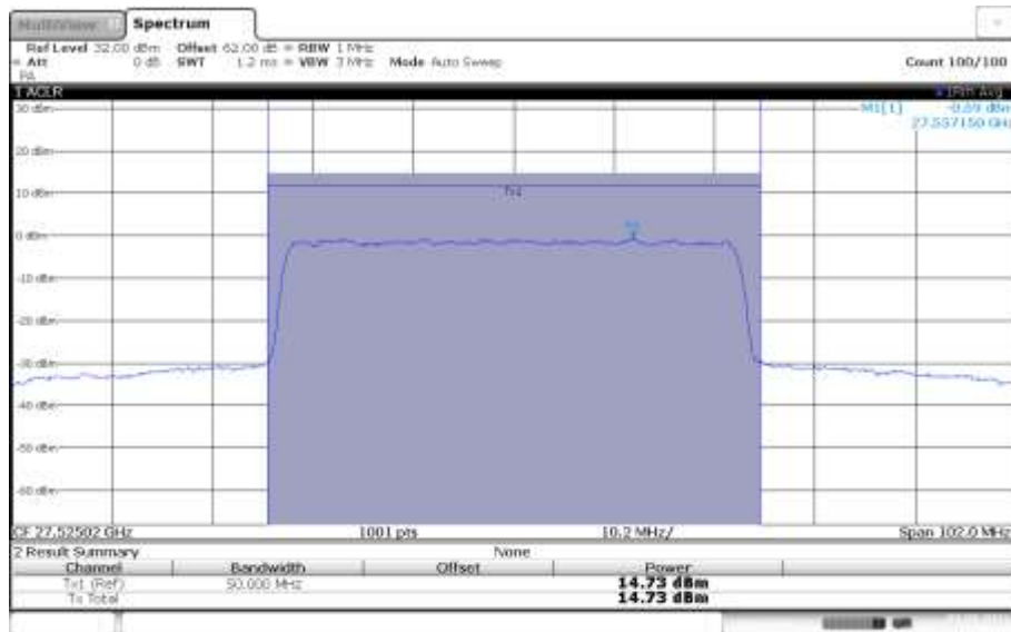
n261, Module0, 50MHz Bandwidth, 100% RB, LOW CHANNEL, QPSK
