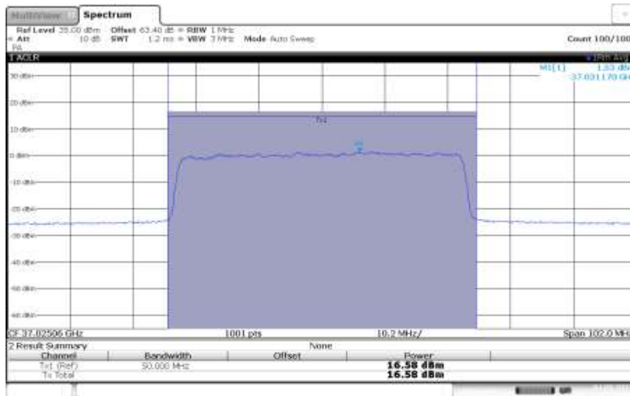
n260, Module0, 50MHz Bandwidth, 100% RB, LOW CHANNEL, QPSK
