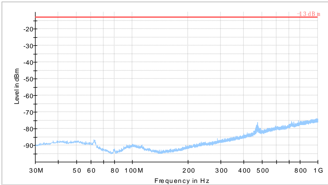
30MHz-1GHz
