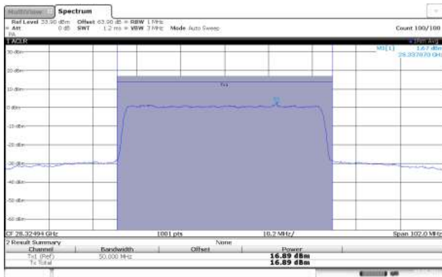
n261, Module0, 50MHz Bandwidth, 100% RB, HIGH CHANNEL, QPSK
