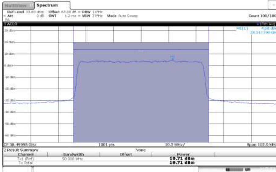
n260, Module1, 50MHz Bandwidth, 100% RB, MID CHANNEL, QPSK
