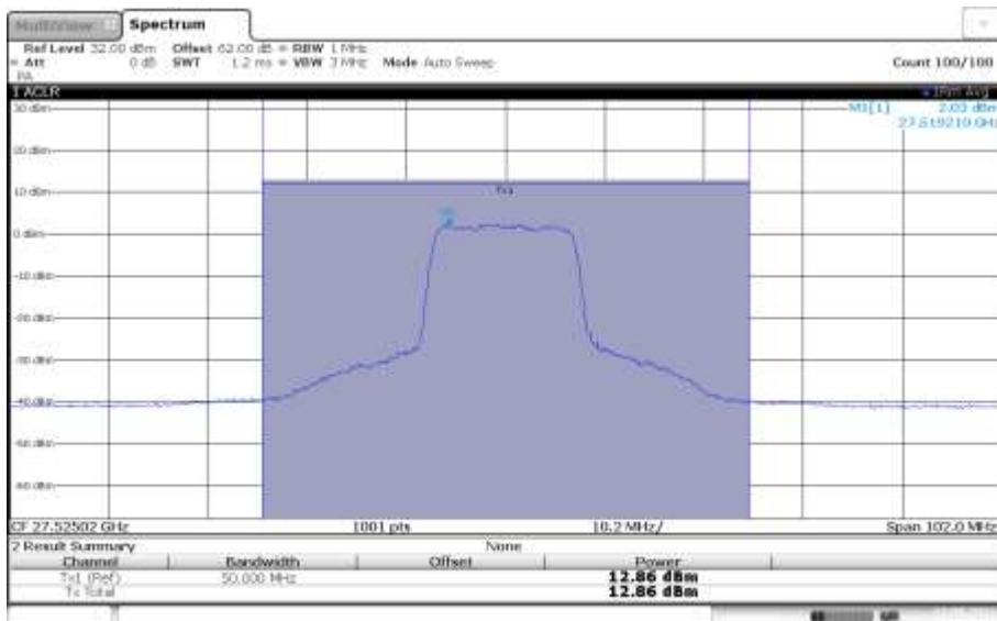
n261, Module1, 50MHz Bandwidth, 10 RB, LOW CHANNEL, QPSK
