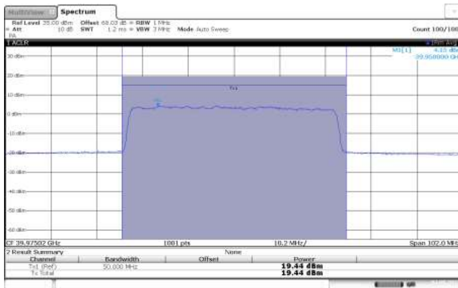
n260, Module0, 50MHz Bandwidth, 100% RB, HIGH CHANNEL, QPSK
