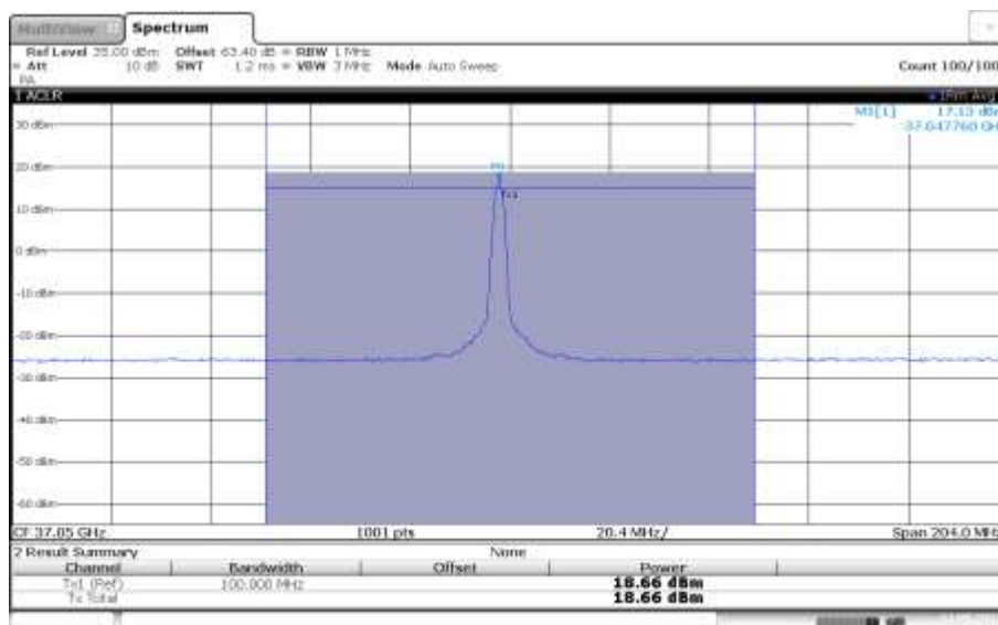
n260, Module1, 100MHz Bandwidth, 1 RB, LOW CHANNEL, QPSK
