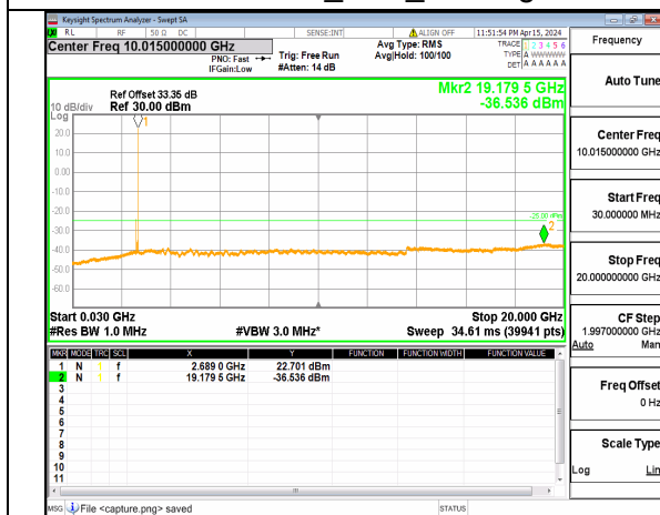
n41 (30MHz-20GHz) 90M DFT-s-OFDM QPSK Inner_1RB_Right High
