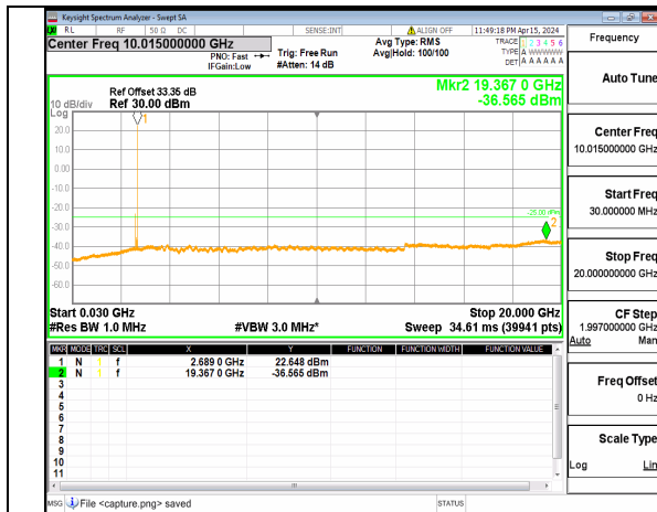
n41 (30MHz-20GHz) 90M DFT-s-OFDM BPSK Inner_1RB_Right High
