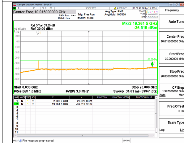
n41 (30MHz-20GHz) 90M DFT-s-OFDM QPSK Inner_1RB_Left High
