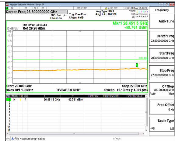
n41 (20GHz-27GHz) 100M DFT-s-OFDM BPSK Inner_1RB_Right Low
