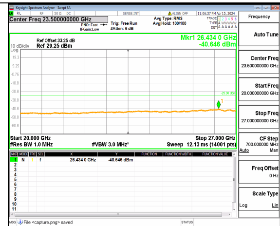
n41 (20GHz-27GHz) 70M DFT-s-OFDM BPSK Inner_1RB_Left Low
