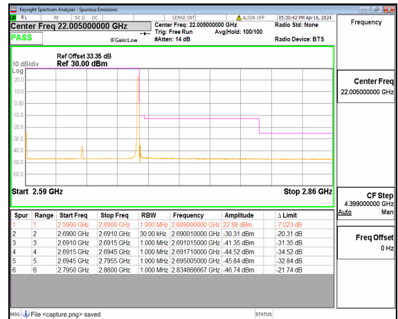
n41 100M DFT-s-OFDM BPSK Edge_1RB_Right High
