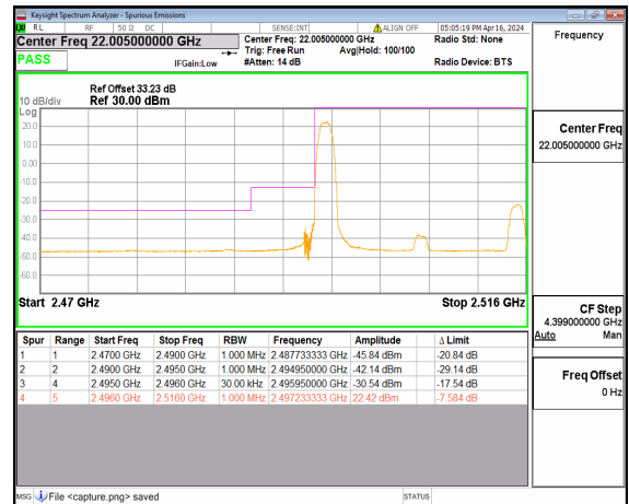
n41 20M DFT-s-OFDM QPSK Edge_1RB_Left Low
