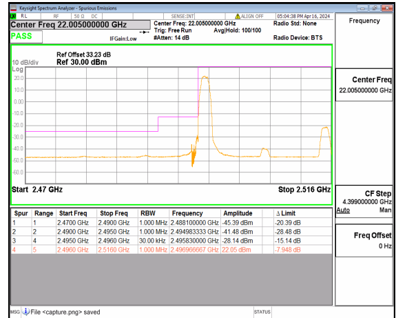
n41 20M DFT-s-OFDM BPSK Edge_1RB_Left Low
