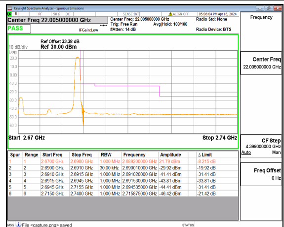
n41 20M DFT-s-OFDM BPSK Edge_1RB_Right High
