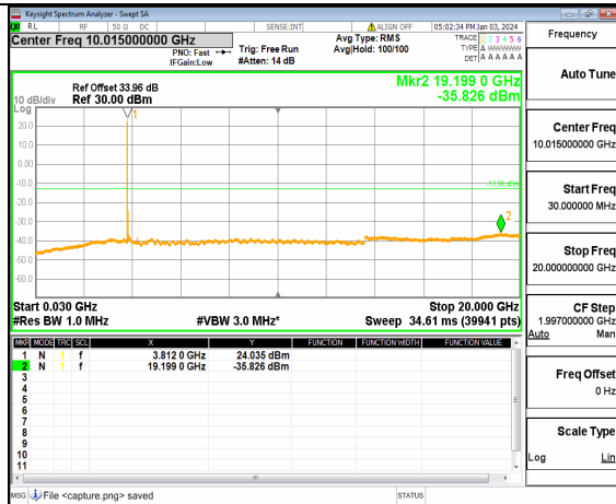
n77(3700-3980MHz) (30MHz-20GHz) 60M DFT-s-OFDM BPSK Inner 1RB Left Mid
