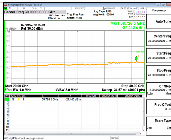
n77(3700-3980MHz) (20GHz-40GHz) 40M DFT-s-OFDM BPSK Inner 1RB Left High
