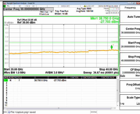
n77(3700-3980MHz) (20GHz-40GHz) 40M DFT-s-OFDM QPSK Inner_1RB Right Mid
