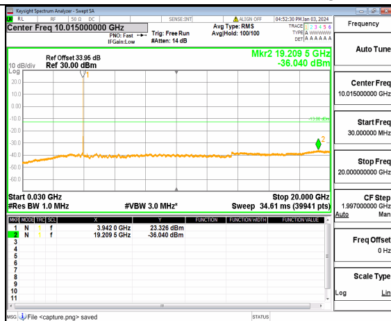
n77(3700-3980MHz) (30MHz-20GHz) 40M DFT-s-OFDM BPSK Inner 1RB Left High
