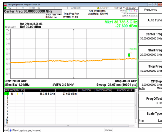
n77(3700-3980MHz) (20GHz-40GHz) 60M DFT-s-OFDM BPSK Inner 1RB Right Mid
