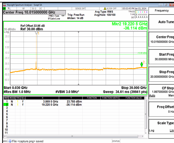
n77(3700-3980MHz) (30MHz-20GHz) 60M DFT-s-OFDM BPSK Inner 1RB Right Mid
