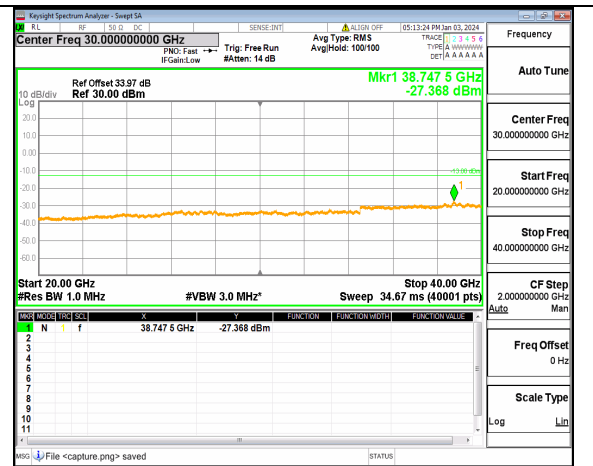
n77(3700-3980MHz) (20GHz-40GHz) 80M DFT-s-OFDM BPSK Inner_1RB_Left Low
