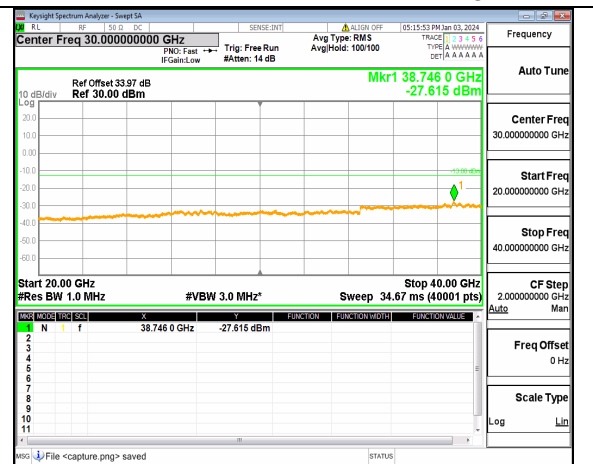
n77(3700-3980MHz) (20GHz-40GHz) 80M DFT-s-OFDM QPSK Inner_1RB_Left Low
