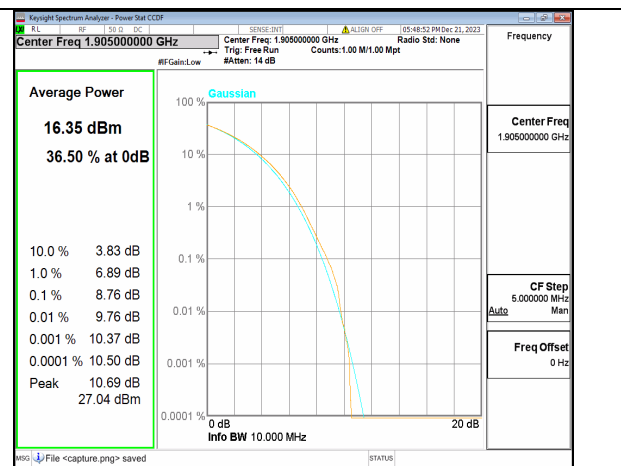
n2 10M CP-OFDM 256QAM Outer_Full High
