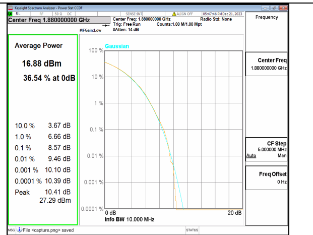
n2 10M CP-OFDM 256QAM Outer_Full Mid
