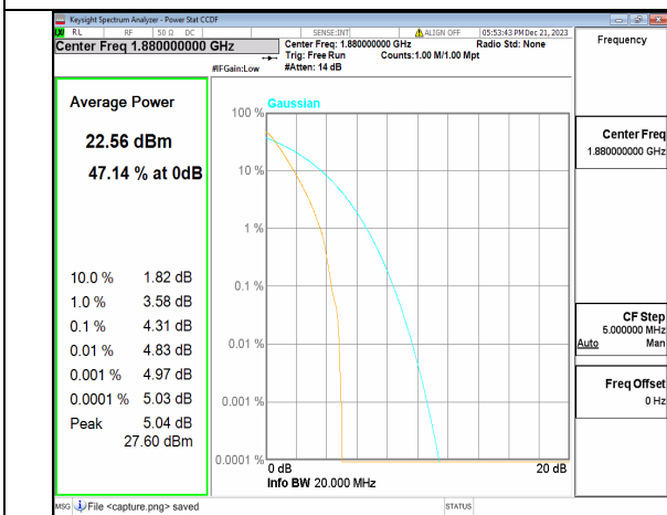
n2 20M DFT-s-OFDM BPSK Outer_Full Mid
