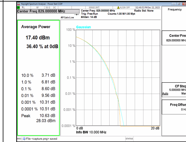
n5 10M CP-OFDM 256QAM Outer_Full Low
