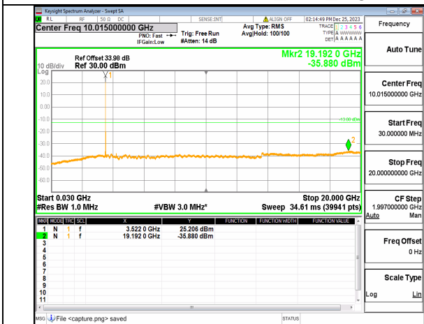
n77(3450-3550MHz) (30MHz-20GHz) 30M DFT-s-OFDM BPSK Inner_1RB_Left High
