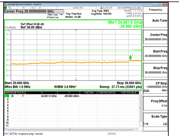
n77(3450-3550MHz) (20GHz-36GHz) 30M DFT-s-OFDM QPSK Inner_1RB_Right Mid
