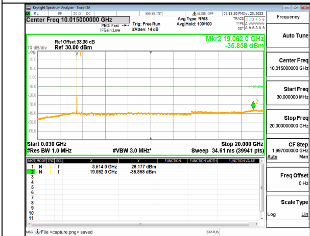
n77(3450-3550MHz) (30MHz-20GHz) 30M DFT-s-OFDM QPSK Inner_1RB_Right Mid
