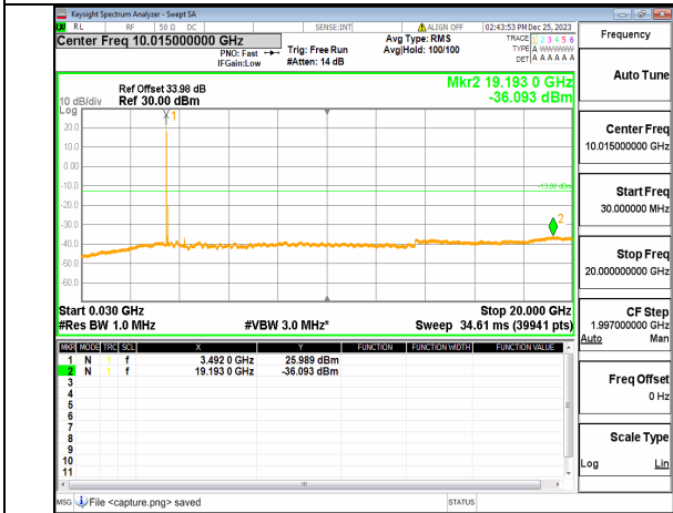
n77(3450-3550MHz) (30MHz-20GHz) 60M DFT-s-OFDM BPSK Inner_1RB_Left High
