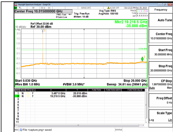
n77(3450-3550MHz) (30MHz-20GHz) 30M DFT-s-OFDM QPSK Inner_1RB_Left Mid
