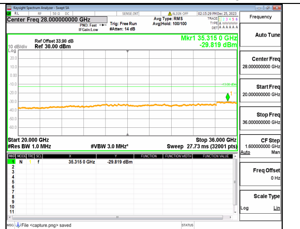
n77(3450-3550MHz) (20GHz-36GHz) 30M DFT-s-OFDM BPSK Inner_1RB_Left High
