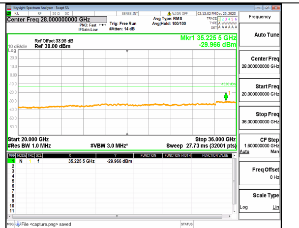
n77(3450-3550MHz) (20GHz-36GHz) 30M DFT-s-OFDM QPSK Inner_1RB_Left Mid
