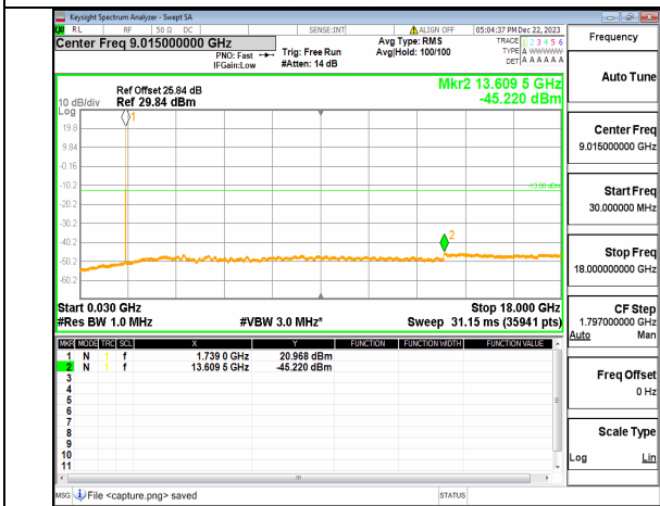
n66 (30MHz-18GHz) 15M DFT-s-OFDM BPSK Inner_1RB_Left Mid
