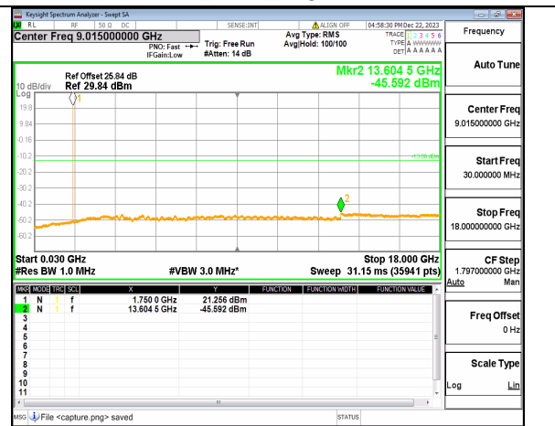
n66 (30MHz-18GHz) 10M DFT-s-OFDM BPSK Inner_1RB_Right Mid
