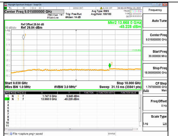
n66 (30MHz-18GHz) 5M DFT-s-OFDM BPSK Inner_1RB_Right Mid
