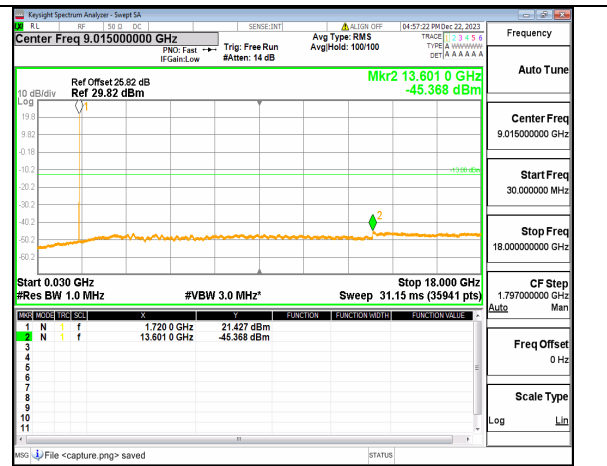
n66 (30MHz-18GHz) 10M DFT-s-OFDM QPSK Inner_1RB_Right Low
