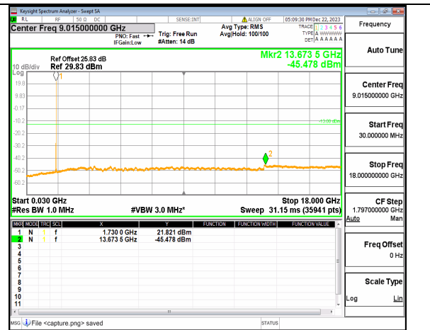
n66 (30MHz-18GHz) 20M DFT-s-OFDM BPSK Inner_1RB_Right Low
