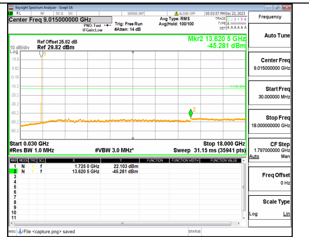
n66 (30MHz-18GHz) 15M DFT-s-OFDM QPSK Inner_1RB_Right Low
