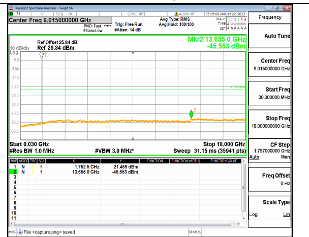
n66 (30MHz-18GHz) 15M DFT-s-OFDM BPSK Inner_1RB_Right Mid
