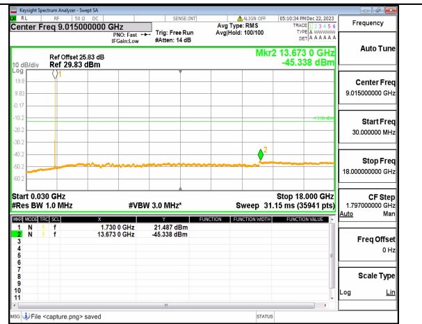
n66 (30MHz-18GHz) 20M DFT-s-OFDM QPSK Inner_1RB_Right Low
