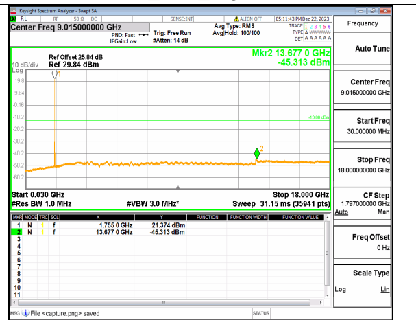
n66 (30MHz-18GHz) 20M DFT-s-OFDM BPSK Inner_1RB_Right Mid
