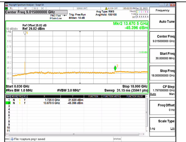
n66 (30MHz-18GHz) 15M DFT-s-OFDM BPSK Inner_1RB_Right Low
