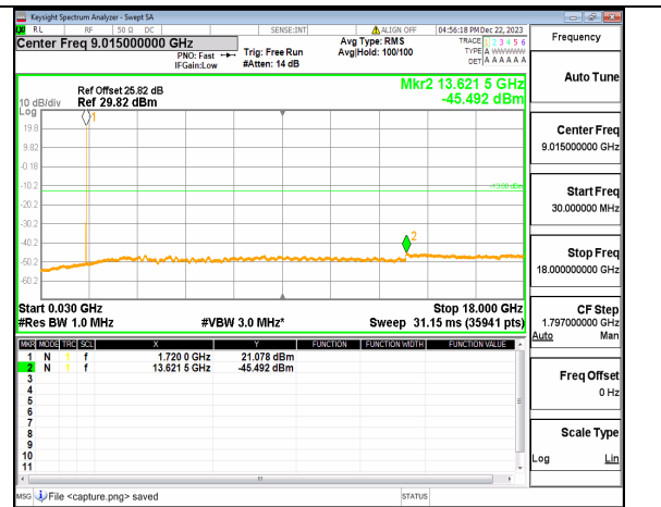
n66 (30MHz-18GHz) 10M DFT-s-OFDM BPSK Inner_1RB_Right Low
