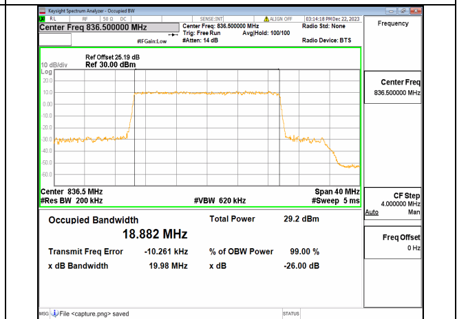
n5 20M CP-OFDM QPSK Outer_Full Mid
