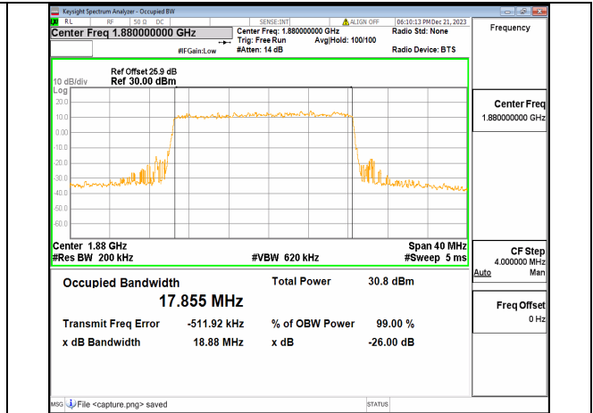
n2 20M DFT-s-OFDM QPSK Outer_Full Mid
