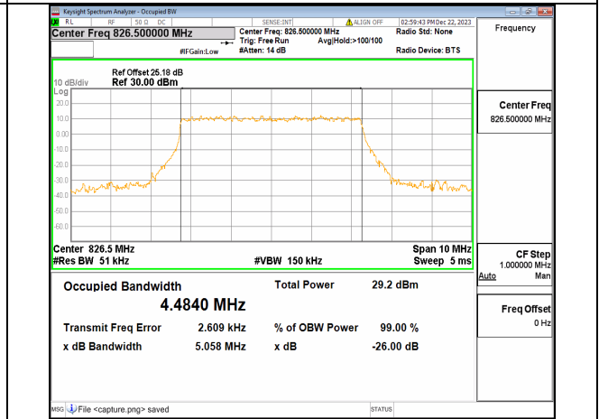
n5 5M DFT-s-OFDM 64QAM Outer_Full Low
