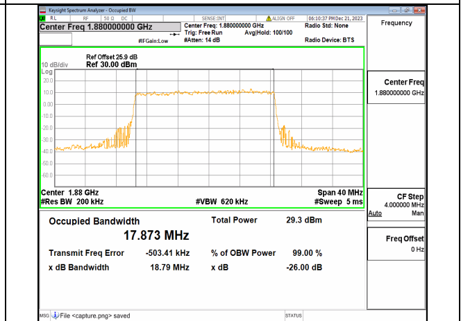
n2 20M DFT-s-OFDM 64QAM Outer_Full Mid
