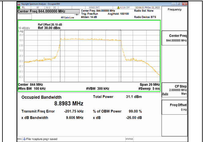
n5 10M DFT-s-OFDM QPSK Outer_Full High
