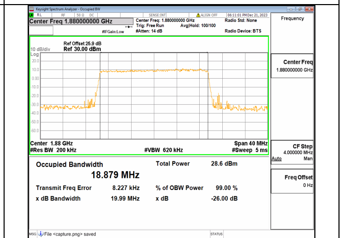
n2 20M CP-OFDM QPSK Outer_Full Mid
