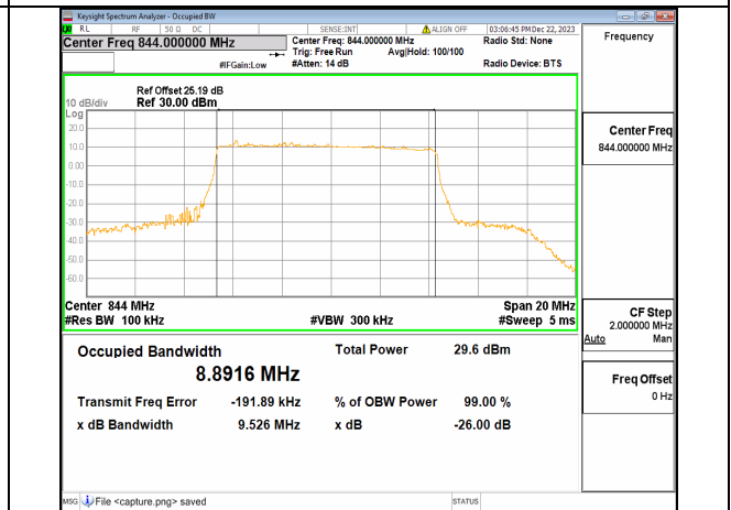
n5 10M DFT-s-OFDM 64QAM Outer_Full High
