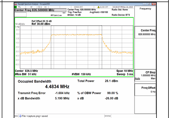
n5 5M CP-OFDM QPSK Outer_Full Low
