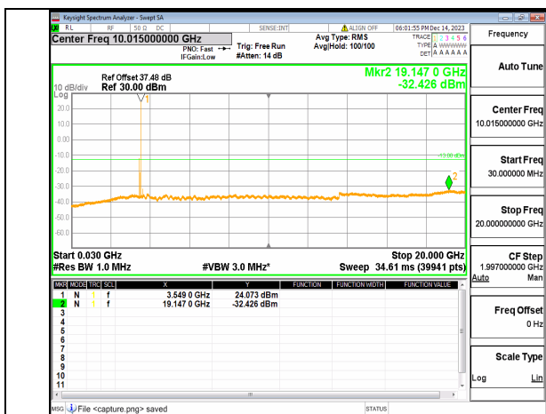
2A_n77(3450-3650MHz) (30MHz-20GHz) 100M DFT-s-OFDM QPSK Inner_1RB_Right Low
