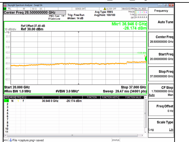
2A_n77(3450-3650MHz) (20GHz-37GHz) 100M DFT-s-OFDM BPSK Inner_1RB_Left Mid
