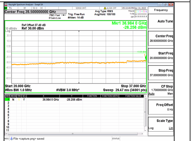
2A_n77(3450-3650MHz) (20GHz-37GHz) 30M DFT-s-OFDM QPSK Inner_1RB_Right Mid
