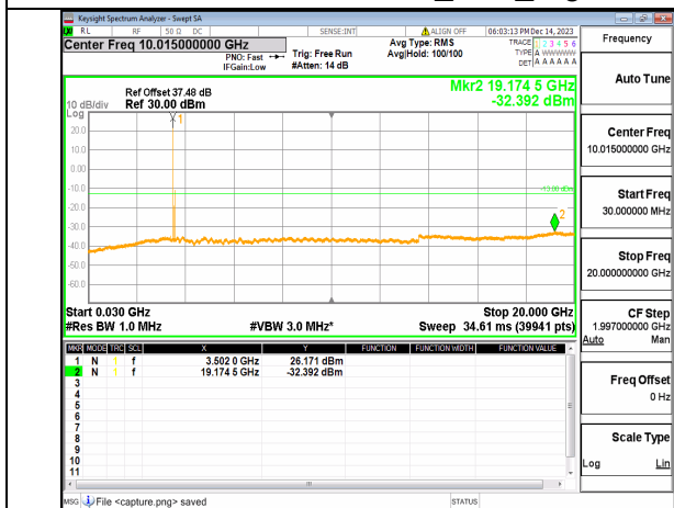
2A_n77(3450-3650MHz) (30MHz-20GHz) 100M DFT-s-OFDM BPSK Inner_1RB_Left Mid
