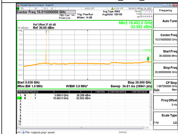
2A_n77(3450-3650MHz) (30MHz-20GHz) 100M DFT-s-OFDM BPSK Inner_1RB_Right Mid
