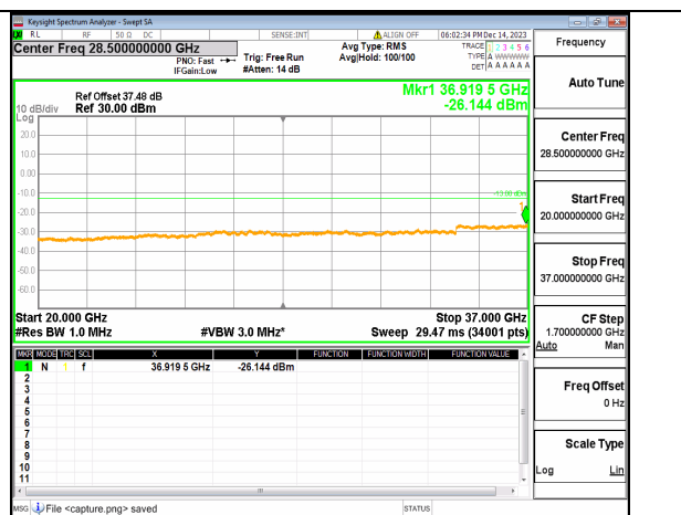
2A_n77(3450-3650MHz) (20GHz-37GHz) 100M DFT-s-OFDM QPSK Inner_1RB_Right Low
