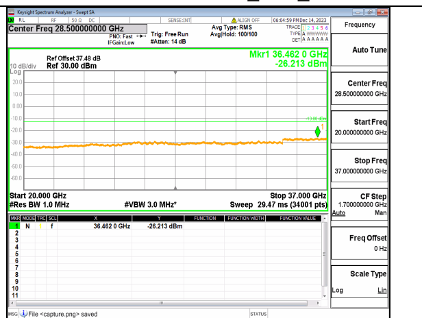
2A_n77(3450-3650MHz) (20GHz-37GHz) 100M DFT-s-OFDM BPSK Inner_1RB_Right Mid
