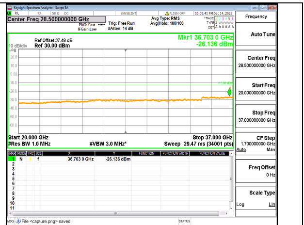
2A_n77(3450-3650MHz) (20GHz-37GHz) 30M DFT-s-OFDM QPSK Inner_1RB_Left Mid
