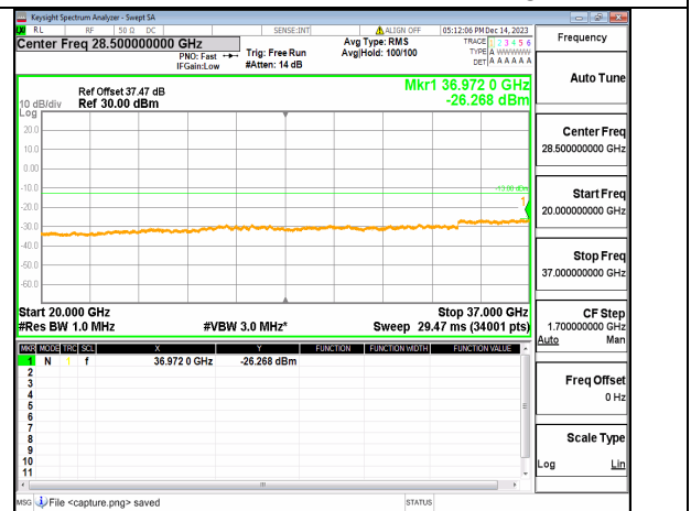
2A_n77(3450-3650MHz) (20GHz-37GHz) 30M DFT-s-OFDM BPSK Inner_1RB_Left High
