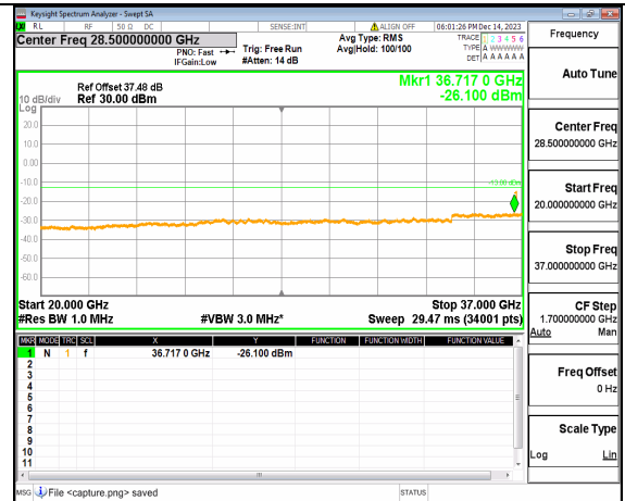
2A_n77(3450-3650MHz) (20GHz-37GHz) 100M DFT-s-OFDM QPSK Inner_1RB_Left Low
