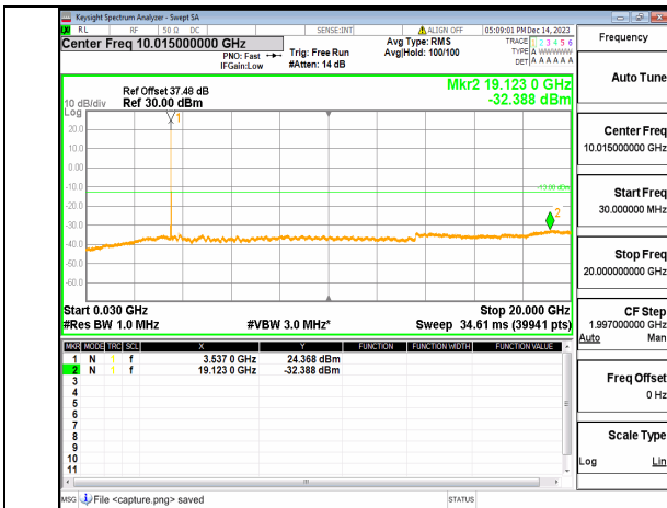
2A_n77(3450-3650MHz) (30MHz-20GHz) 30M DFT-s-OFDM QPSK Inner_1RB_Left Mid
