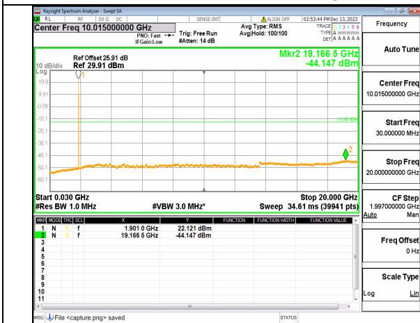
5A_n2 (30MHz-20GHz) 10M DFT-s-OFDM QPSK Inner_1RB_Left High
