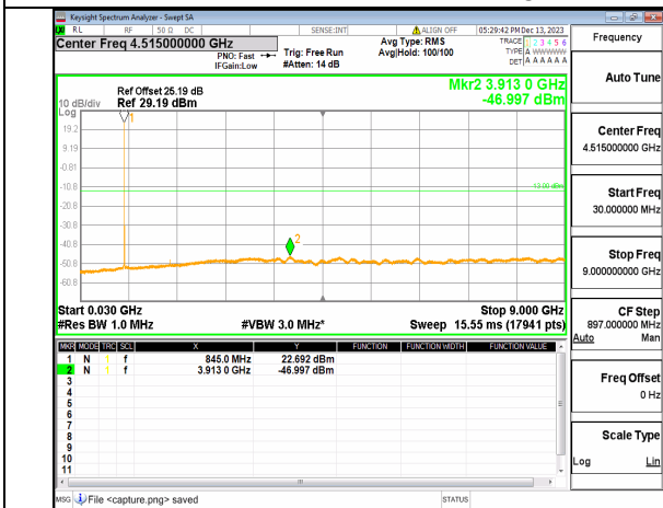
66A_n5 (30MHz-9GHz) 5M DFT-s-OFDM QPSK Inner_1RB_Left High
