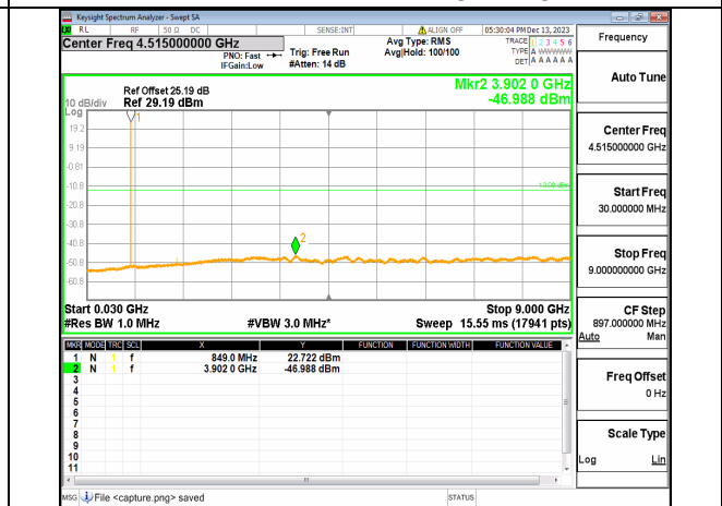
66A_n5 (30MHz-9GHz) 5M DFT-s-OFDM QPSK Inner_1RB_Right High
