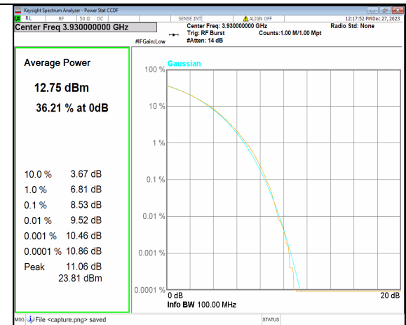
2A_n77(3700-3980MHz) 100M CP-OFDM 256QAM Outer_Full High
