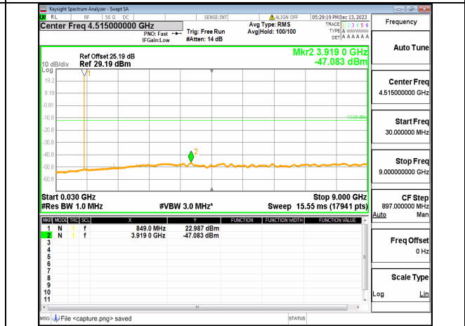
66A_n5 (30MHz-9GHz) 5M DFT-s-OFDM BPSK Inner_1RB_Right High
