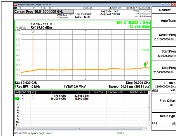
5A_n2 (30MHz-20GHz) 5M DFT-s-OFDM QPSK Inner_1RB_Left Mid
