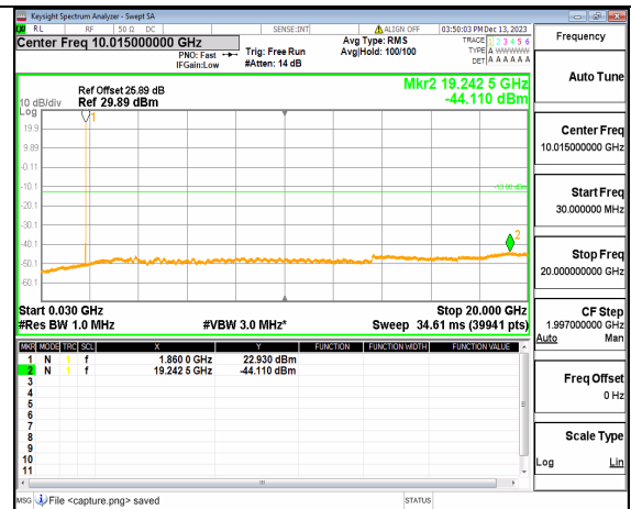
5A_n2 (30MHz-20GHz) 10M DFT-s-OFDM QPSK Inner_1RB_Right Low
