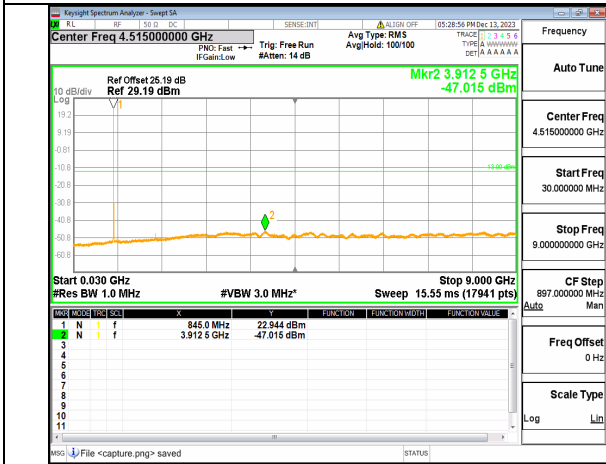
66A_n5 (30MHz-9GHz) 5M DFT-s-OFDM BPSK Inner_1RB_Left High
