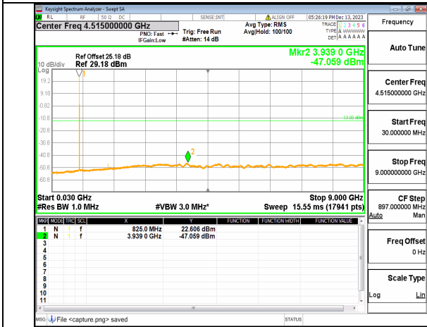
66A_n5 (30MHz-9GHz) 5M DFT-s-OFDM QPSK Inner_1RB_Left Low
