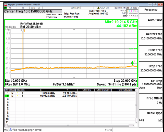
5A_n2 (30MHz-20GHz) 10M DFT-s-OFDM BPSK Inner_1RB_Right Low
