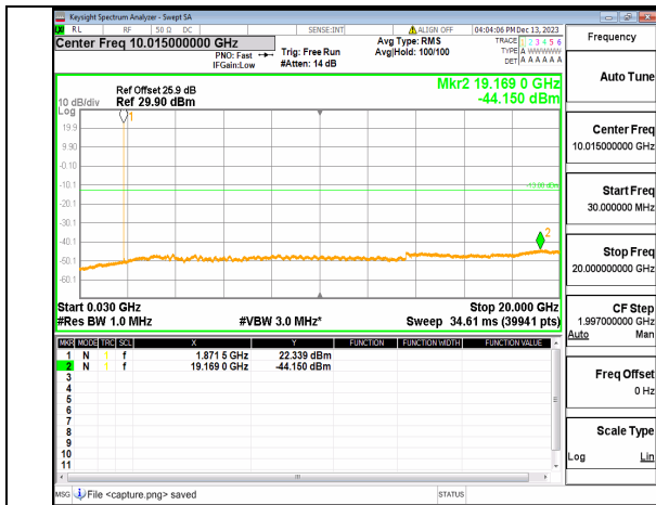
5A_n2 (30MHz-20GHz) 20M DFT-s-OFDM QPSK Inner_1RB_Left Mid
