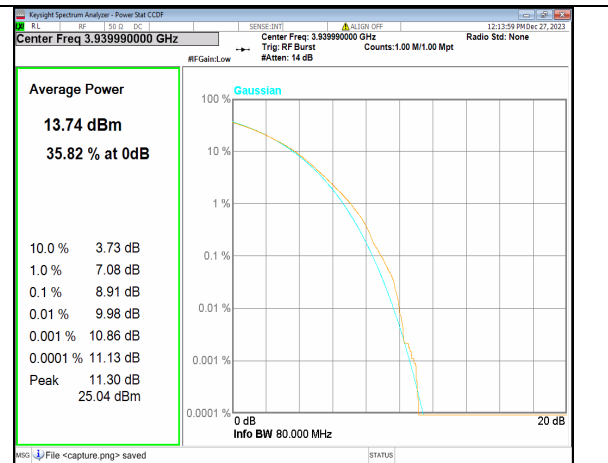
2A_n77(3700-3980MHz) 80M CP-OFDM 256QAM Outer_Full High
