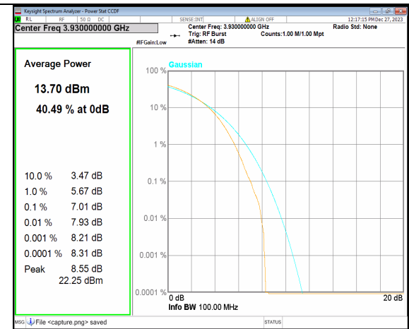
2A_n77(3700-3980MHz) 100M DFT-s-OFDM 256QAM Outer_Full High
