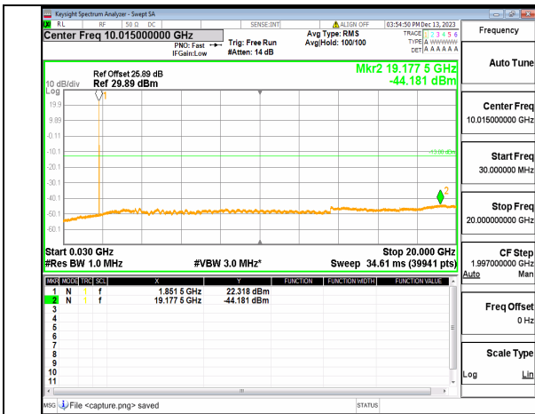
5A_n2 (30MHz-20GHz) 15M DFT-s-OFDM BPSK Inner_1RB_Left Low
