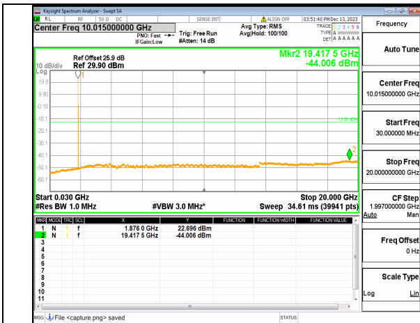
5A_n2 (30MHz-20GHz) 10M DFT-s-OFDM QPSK Inner_1RB_Left Mid
