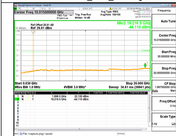
5A_n2 (30MHz-20GHz) 15M DFT-s-OFDM QPSK Inner_1RB_Left High
