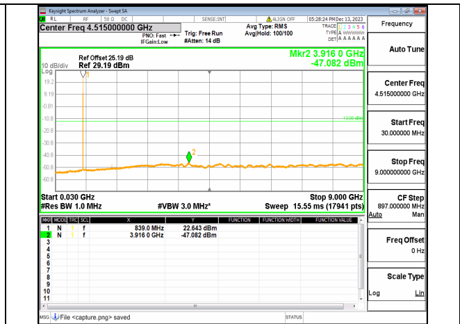
66A_n5 (30MHz-9GHz) 5M DFT-s-OFDM QPSK Inner_1RB_Right Mid
