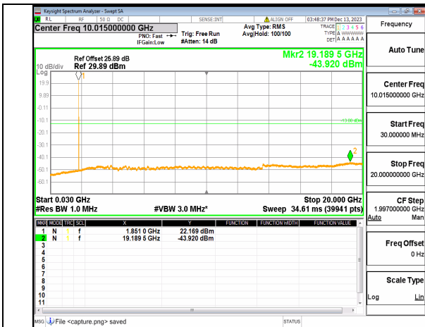
5A_n2 (30MHz-20GHz) 10M DFT-s-OFDM BPSK Inner_1RB_Left Low
