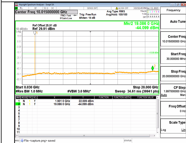
5A_n2 (30MHz-20GHz) 10M DFT-s-OFDM BPSK Inner_1RB_Left High
