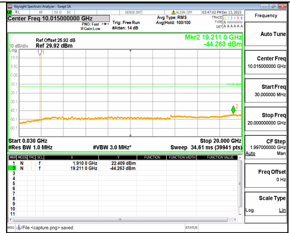
5A_n2 (30MHz-20GHz) 5M DFT-s-OFDM BPSK Inner_1RB_Right High
