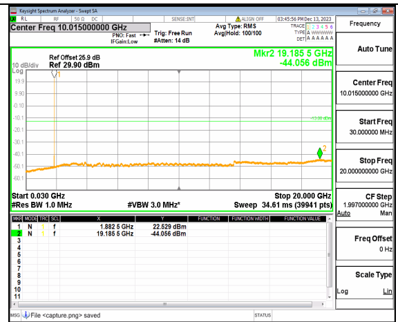
5A_n2 (30MHz-20GHz) 5M DFT-s-OFDM QPSK Inner_1RB_Right Mid
