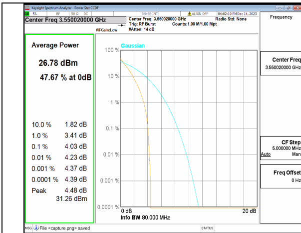
2A_n77(3450-3650MHz) 80M DFT-s-OFDM BPSK Outer_Full Mid
