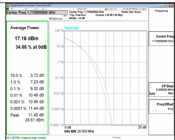
2A_n66 20M CP-OFDM 256QAM Outer_Full High
