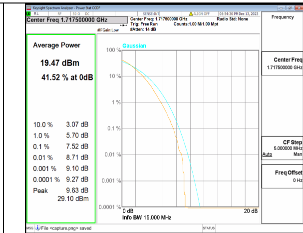
2A_n66 15M DFT-s-OFDM 256QAM Outer_Full Low
