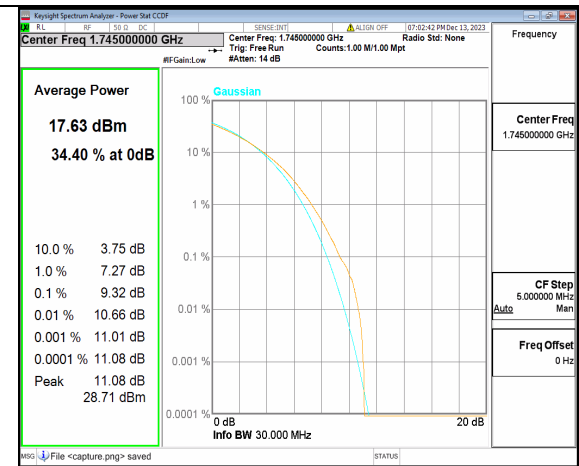
2A_n66 30M CP-OFDM 256QAM Outer_Full Mid
