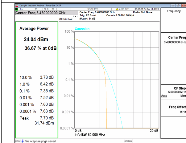
2A_n77(3450-3650MHz) 60M CP-OFDM QPSK Outer_Full Low
