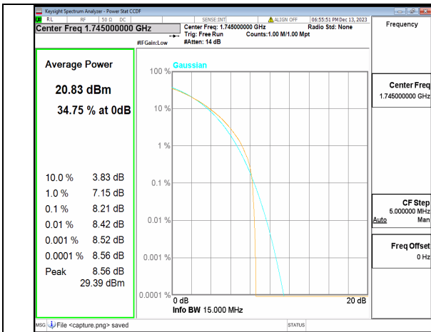
2A_n66 15M CP-OFDM QPSK Outer_Full Mid
