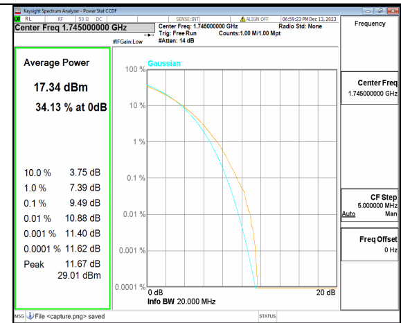
2A_n66 20M CP-OFDM 256QAM Outer_Full Mid
