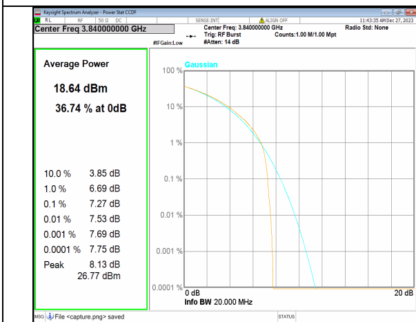
2A_n77(3700-3980MHz) 20M CP-OFDM QPSK Outer_Full Mid
