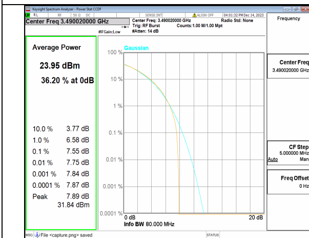
2A_n77(3450-3650MHz) 80M CP-OFDM QPSK Outer_Full Low
