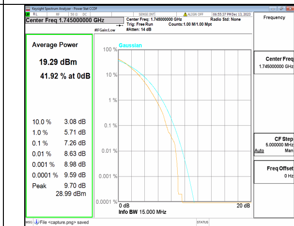
2A_n66 15M DFT-s-OFDM 256QAM Outer_Full Mid
