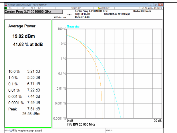
2A_n77(3700-3980MHz) 20M DFT-s-OFDM 256QAM Outer_Full Low
