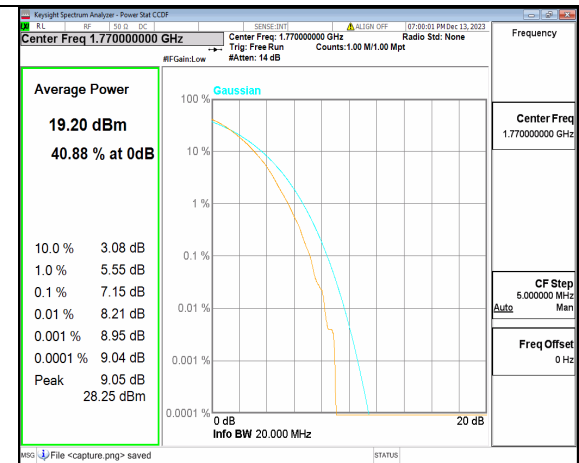
2A_n66 20M DFT-s-OFDM 256QAM Outer_Full High
