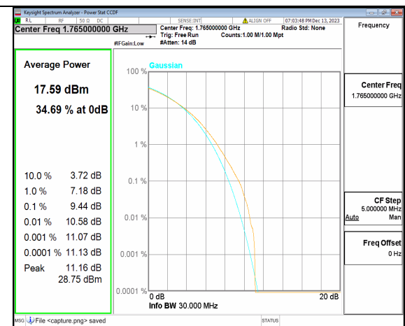
2A_n66 30M CP-OFDM 256QAM Outer_Full High
