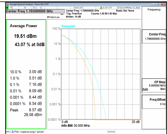
2A_n66 30M DFT-s-OFDM 256QAM Outer_Full High
