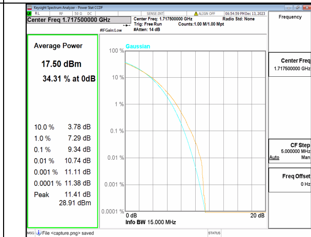
2A_n66 15M CP-OFDM 256QAM Outer_Full Low
