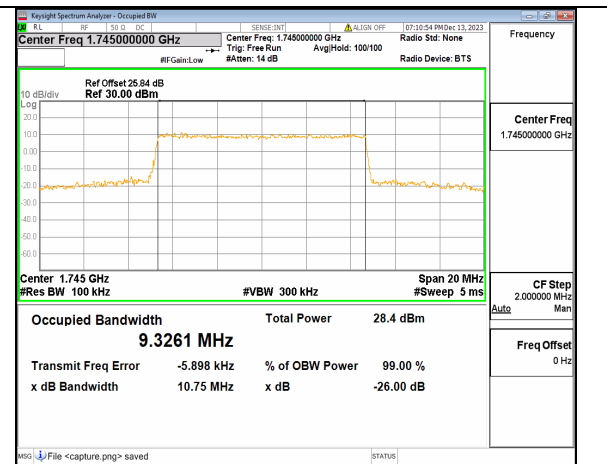
2A_n66 10M CP-OFDM QPSK Outer_Full Mid
