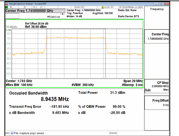
2A_n66 10M DFT-s-OFDM QPSK Outer_Full Mid
