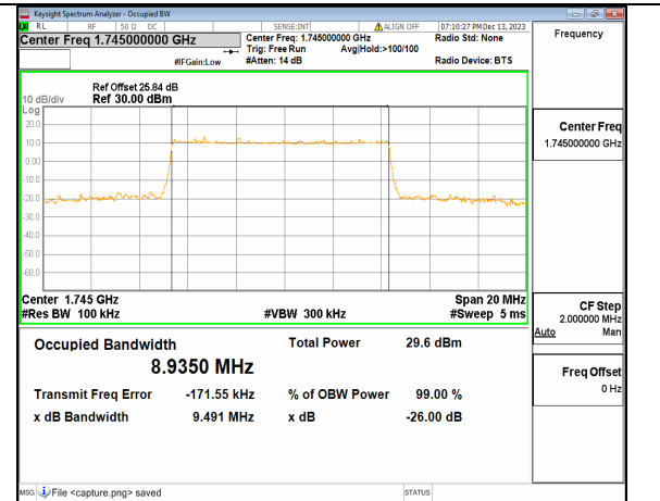
2A_n66 10M DFT-s-OFDM 64QAM Outer_Full Mid
