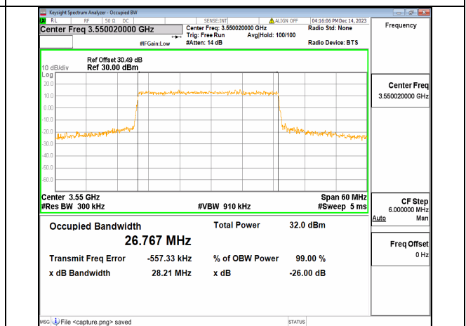
2A_n77(3450-3650MHz) 30M CP-OFDM QPSK Outer_Full Mid
