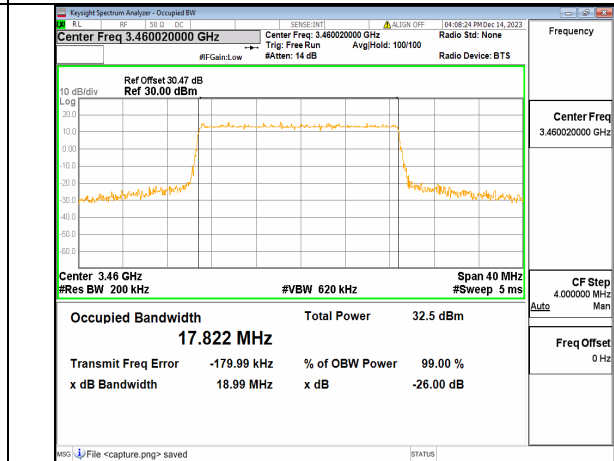
2A_n77(3450-3650MHz) 20M DFT-s-OFDM 64QAM Outer_Full Low
