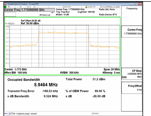
2A_n66 10M DFT-s-OFDM QPSK Outer_Full High
