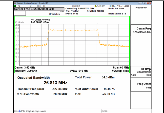
2A_n77(3450-3650MHz) 30M DFT-s-OFDM QPSK Outer_Full Mid
