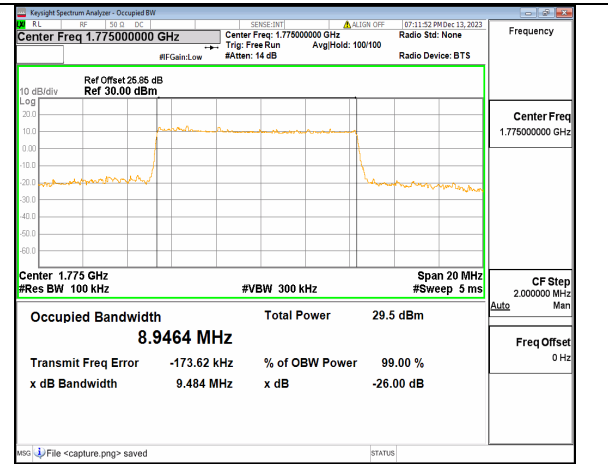
2A_n66 10M DFT-s-OFDM 64QAM Outer_Full High
