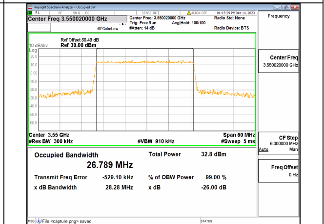
2A_n77(3450-3650MHz) 30M DFT-s-OFDM 64QAM Outer_Full Mid
