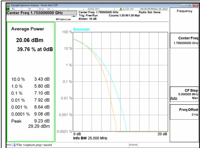
66C / 20+5MHz / Mid CH / 64QAM
