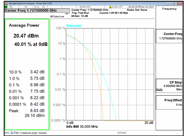
66C / 20+15MHz / Low CH / 64QAM
