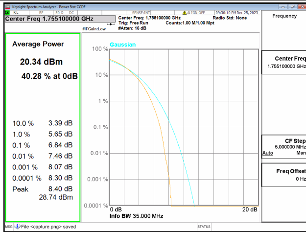
66C / 20+15MHz / Mid CH / 16QAM
