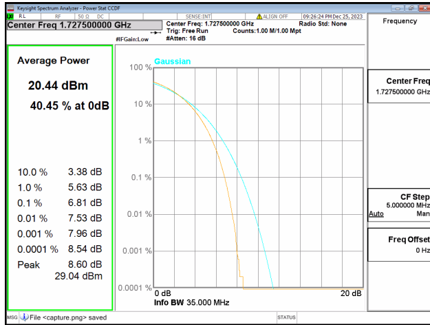
66C / 20+15MHz / Low CH / 16QAM
