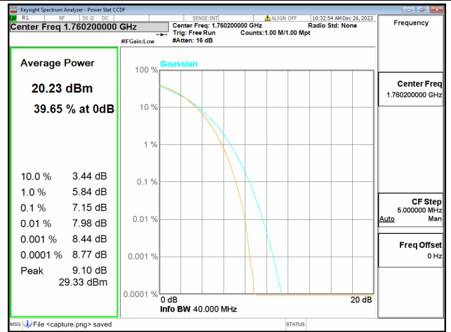
66C / 20+20MHz / High CH / 64QAM
