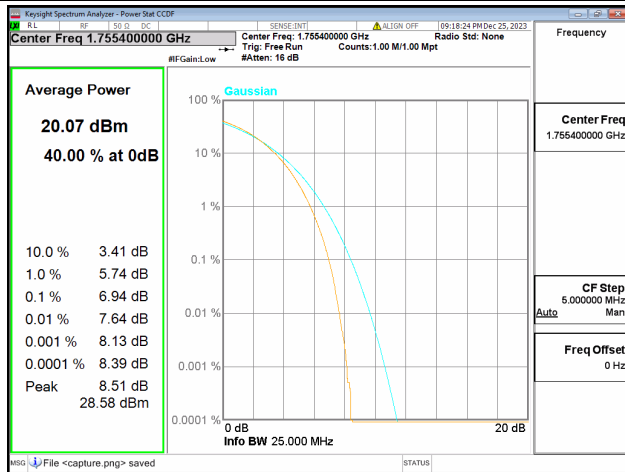
66C / 10+15MHz / Mid CH / 16QAM
