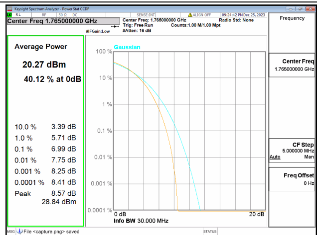
66C / 15+15MHz / High CH / 16QAM
