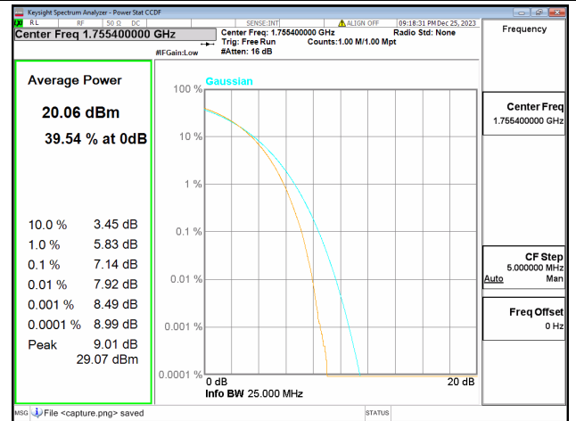
66C / 10+15MHz / Mid CH / 64QAM
