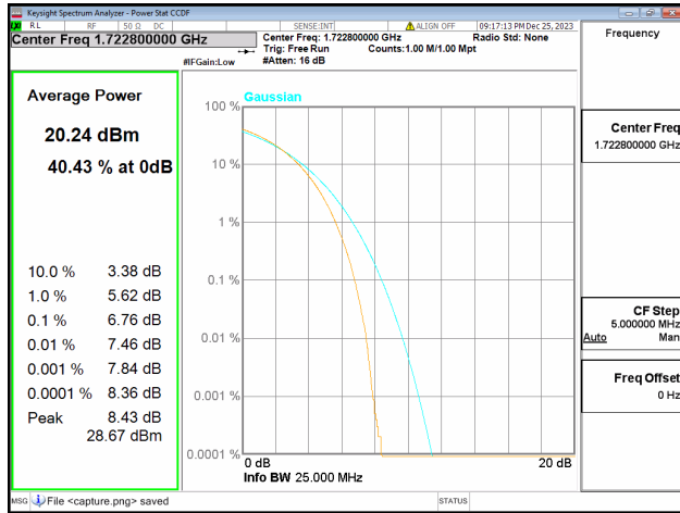
66C / 10+15MHz / Low CH / 16QAM
