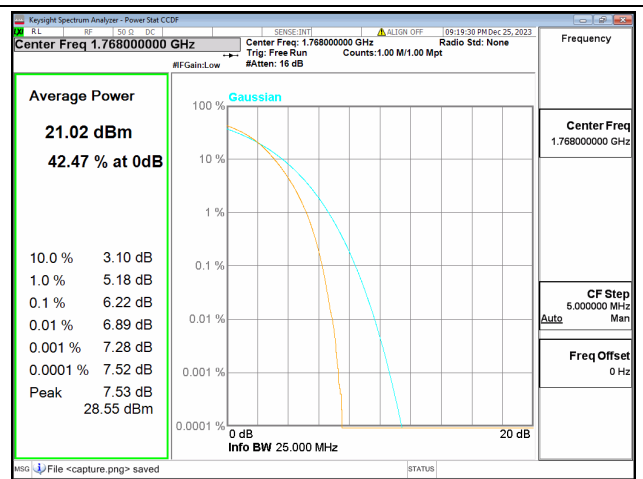
66C / 10+15MHz / High CH / QPSK
