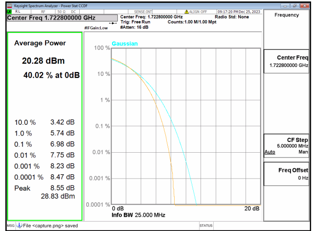
66C / 10+15MHz / Low CH / 64QAM
