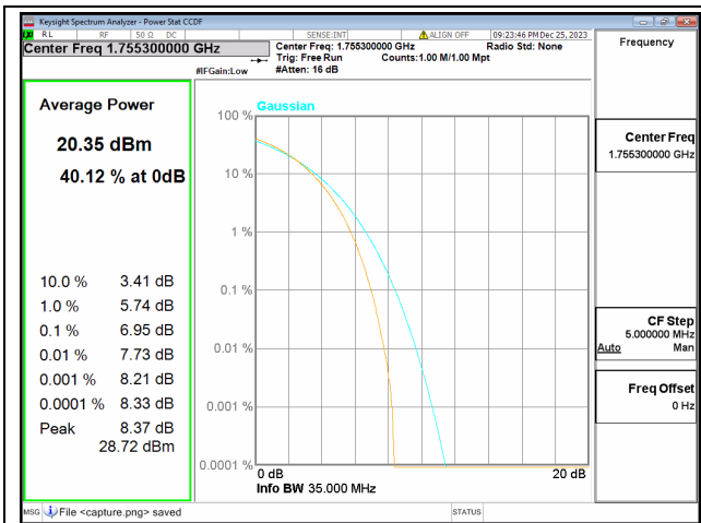
66C / 15+20MHz / Mid CH / 64QAM
