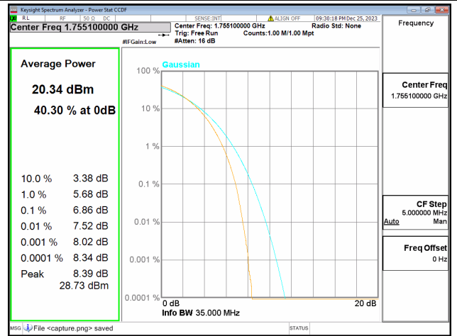
66C / 20+15MHz / Mid CH / 64QAM
