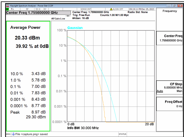
66C / 10+20MHz / Mid CH / 64QAM
