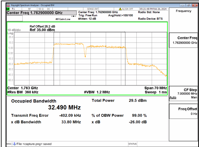
66C / 15+20MHz / 16QAM/ High CH
