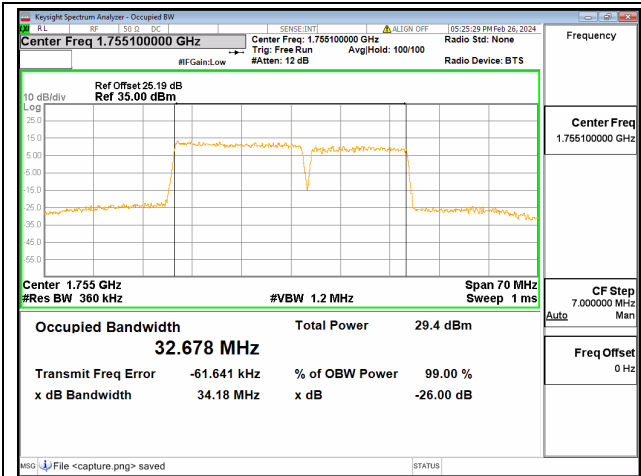
66C / 20+15MHz / 16QAM/ Mid CH
