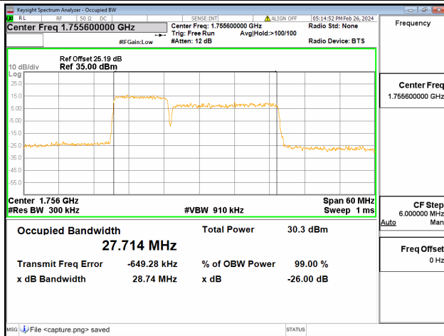
66C / 10+20MHz / QPSK/ Mid CH
