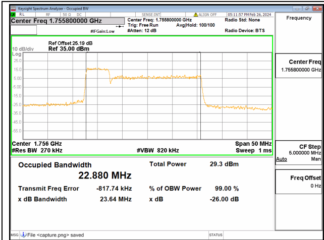
66C / 5+20MHz / 16QAM/ Mid CH
