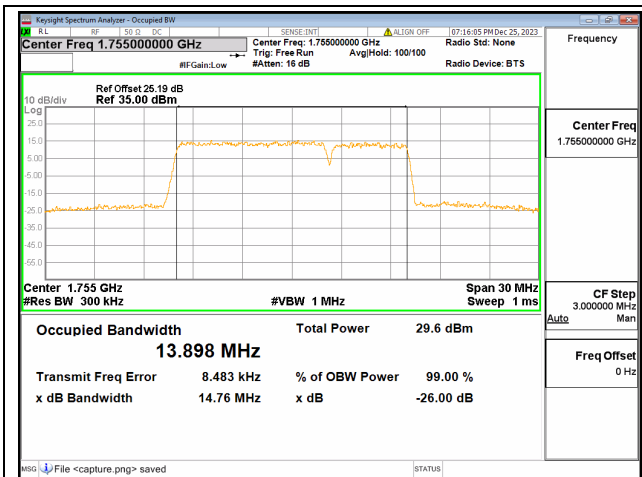
66B / 10+5MHz / 16QAM/ Mid CH
