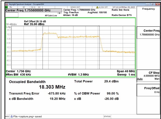
66B / 5+15MHz / 16QAM/ Mid CH
