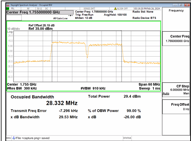
66C / 15+15MHz / 16QAM/ Mid CH
