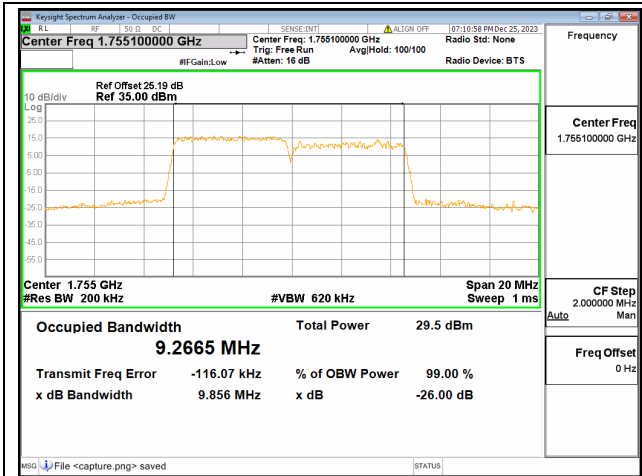
66B / 5+5MHz / 16QAM/ Mid CH
