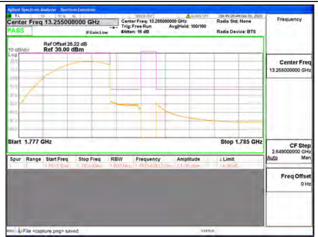
B66 / 1.4MHz / High CH / QPSK / FULL RB
