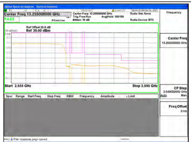
B7 / 20MHz / High CH / QPSK / FULL RB
