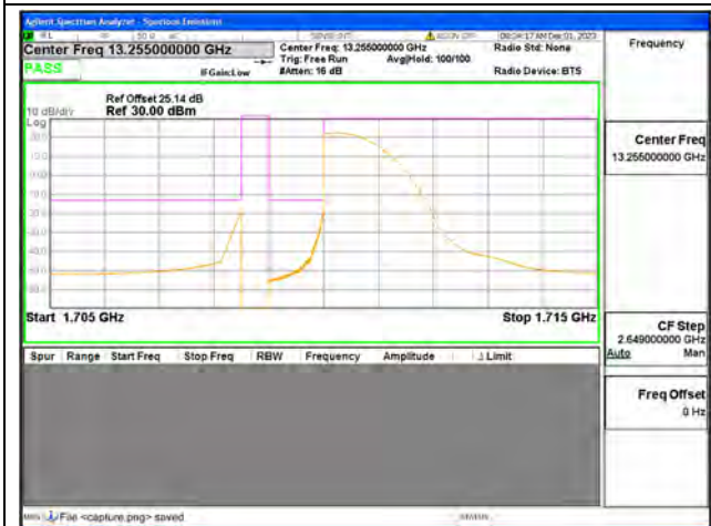
B4 / 3MHz / Low CH / QPSK / 1 RB
