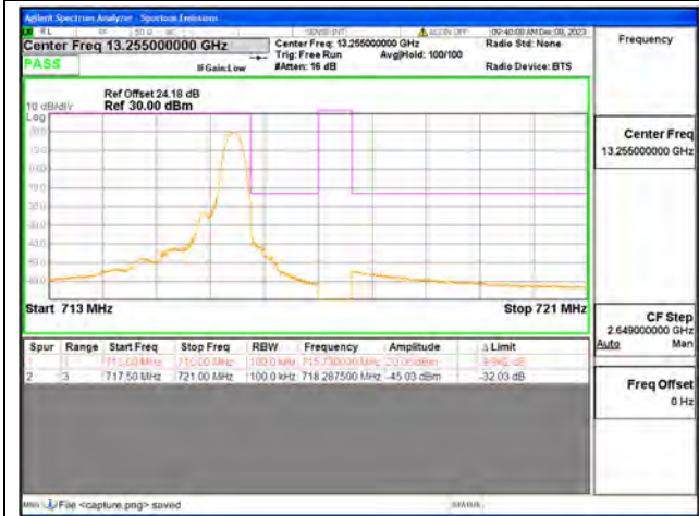
B12 / 1.4MHz / High CH / QPSK / 1 RB
