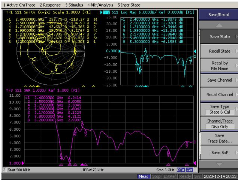
ANT7
