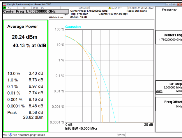
66C / 20+20MHz / High CH / 16QAM
