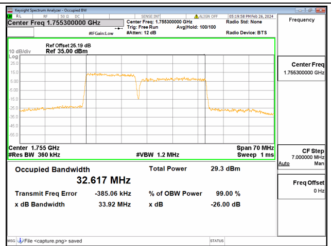
66C / 15+20MHz / 16QAM/ Mid CH
