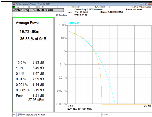
2A_n77(3700-3980MHz) 60M CP-OFDM QPSK Outer_Full Low
