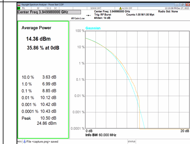
2A_n77(3700-3980MHz) 60M CP-OFDM 256QAM Outer_Full High
