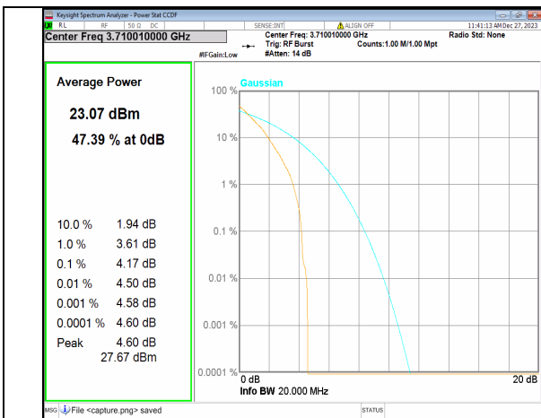
2A_n77(3700-3980MHz) 20M DFT-s-OFDM BPSK Outer_Full Low
