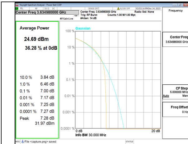
2A_n77(3450-3650MHz) 30M CP-OFDM QPSK Outer_Full High
