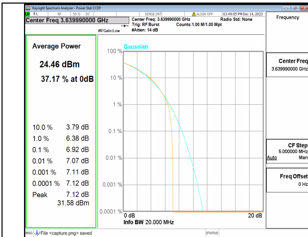
2A_n77(3450-3650MHz) 20M CP-OFDM QPSK Outer_Full High
