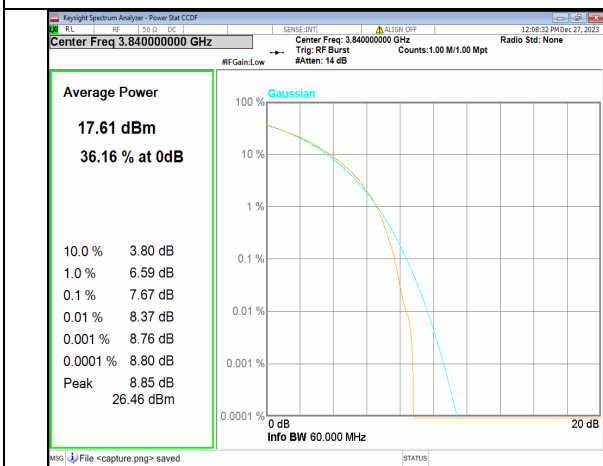
2A_n77(3700-3980MHz) 60M CP-OFDM QPSK Outer_Full Mid
