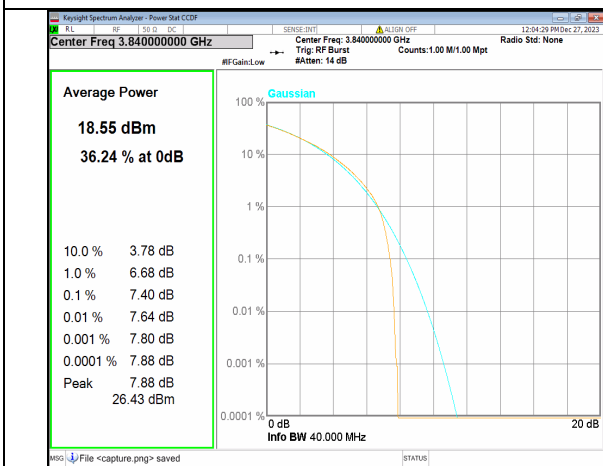
2A_n77(3700-3980MHz) 40M CP-OFDM QPSK Outer_Full Mid
