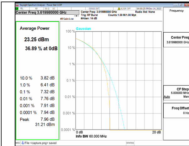
2A_n77(3450-3650MHz) 60M CP-OFDM QPSK Outer_Full High
