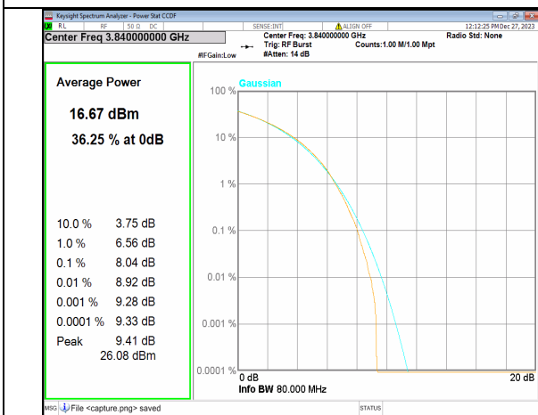
2A_n77(3700-3980MHz) 80M CP-OFDM QPSK Outer_Full Mid
