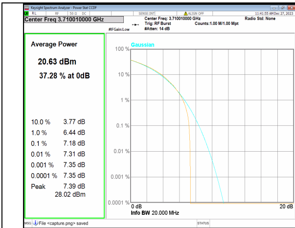
2A_n77(3700-3980MHz) 20M CP-OFDM QPSK Outer_Full Low
