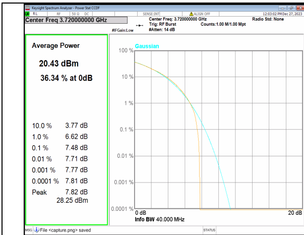
2A_n77(3700-3980MHz) 40M CP-OFDM QPSK Outer_Full Low
