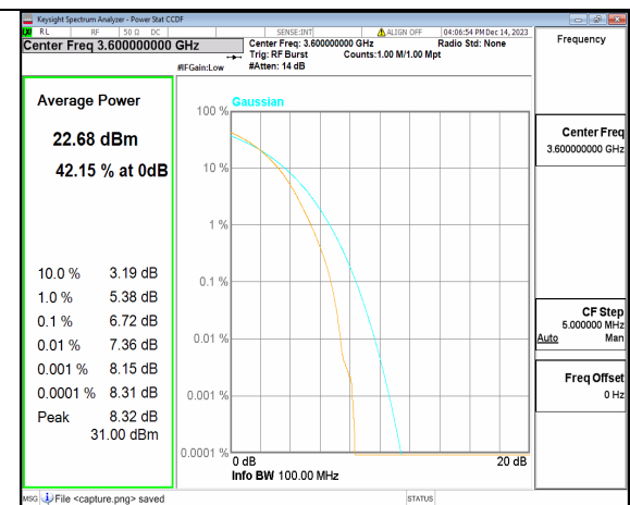
2A_n77(3450-3650MHz) 100M DFT-s-OFDM 256QAM Outer_Full High
