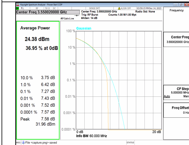
2A_n77(3450-3650MHz) 60M CP-OFDM QPSK Outer_Full Mid
