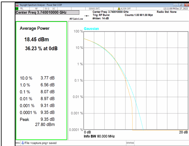
2A_n77(3700-3980MHz) 80M CP-OFDM QPSK Outer_Full Low
