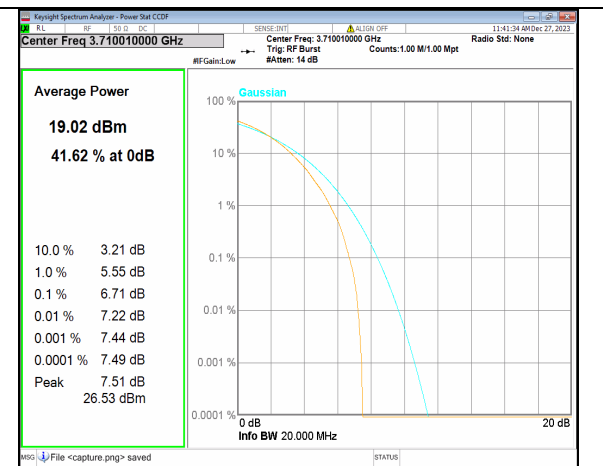
2A_n77(3700-3980MHz) 20M DFT-s-OFDM 256QAM Outer_Full Low
