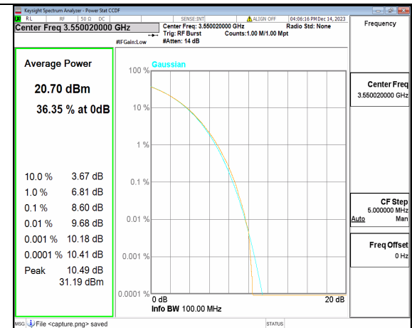
2A_n77(3450-3650MHz) 100M CP-OFDM 256QAM Outer_Full Mid
