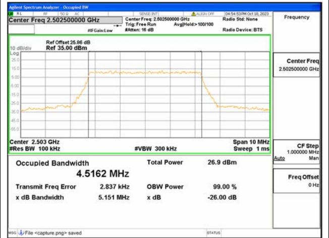
B7 / 5MHz / 256QAM/ Low CH
