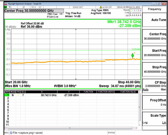
5A_n77(3700-3980MHz) (20GHz-40GHz) 80M DFT-s-OFDM BPSK Outer_Full Mid
