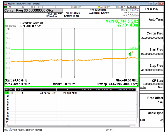
5A_n77(3700-3980MHz) (20GHz-40GHz) 80M DFT-s-OFDM BPSK Edge_1RB_Right Low
