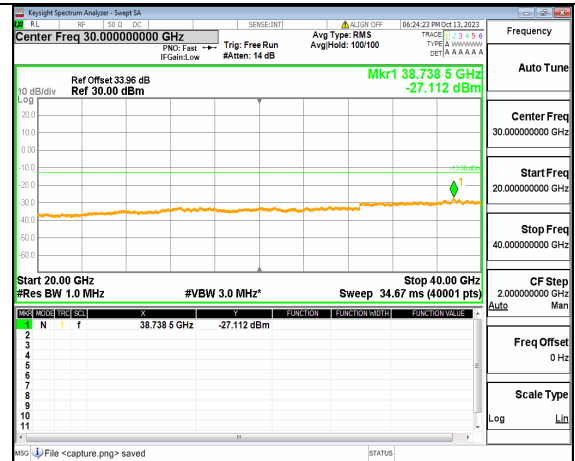
5A_n77(3700-3980MHz) (20GHz-40GHz) 100M DFT-s-OFDM BPSK Edge_1RB_Right Low
