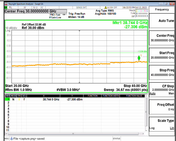
5A_n77(3700-3980MHz) (20GHz-40GHz) 100M DFT-s-OFDM QPSK Outer_Full Mid
