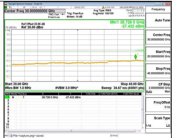
5A_n77(3700-3980MHz) (20GHz-40GHz) 90M DFT-s-OFDM QPSK Edge_1RB_Left High
