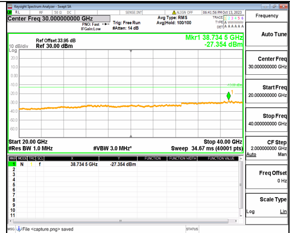
5A_n77(3700-3980MHz) (20GHz-40GHz) 100M DFT-s-OFDM QPSK Outer_Full High
