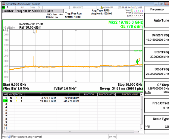
5A_n77(3700-3980MHz) (30MHz-20GHz) 80M DFT-s-OFDM QPSK Edge_1RB_Right Low
