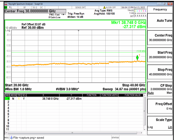
5A_n77(3700-3980MHz) (20GHz-40GHz) 90M DFT-s-OFDM QPSK Edge_1RB_Right Low
