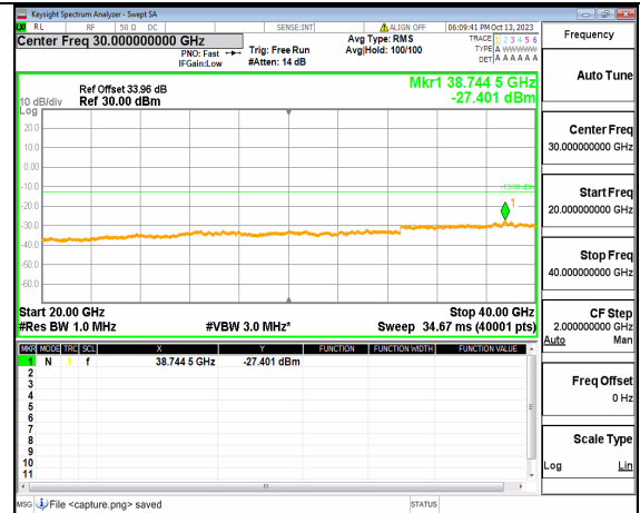
5A_n77(3700-3980MHz) (20GHz-40GHz) 90M DFT-s-OFDM QPSK Outer_Full Mid
