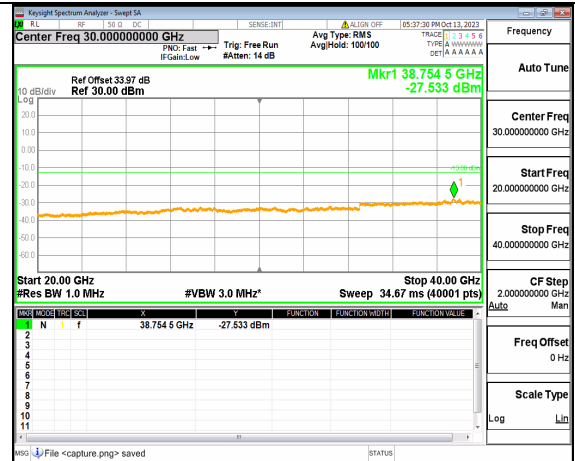
5A_n77(3700-3980MHz) (20GHz-40GHz) 80M DFT-s-OFDM QPSK Outer_Full Low
