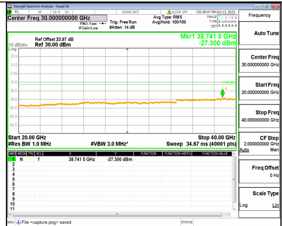
5A_n77(3700-3980MHz) (20GHz-40GHz) 80M DFT-s-OFDM QPSK Edge_1RB_Left Low
