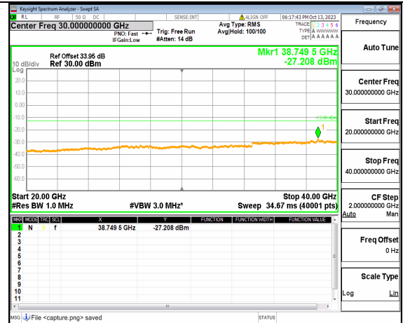
5A_n77(3700-3980MHz) (20GHz-40GHz) 90M DFT-s-OFDM QPSK Outer_Full High
