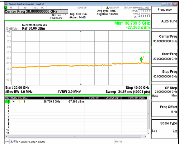
5A_n77(3700-3980MHz) (20GHz-40GHz) 80M DFT-s-OFDM BPSK Edge_1RB_Left Low
