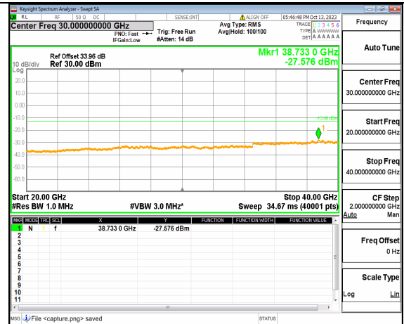
5A_n77(3700-3980MHz) (20GHz-40GHz) 80M DFT-s-OFDM QPSK Edge_1RB_Left Mid
