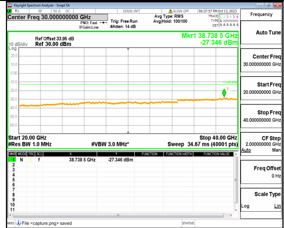
5A_n77(3700-3980MHz) (20GHz-40GHz) 100M DFT-s-OFDM BPSK Outer_Full High
