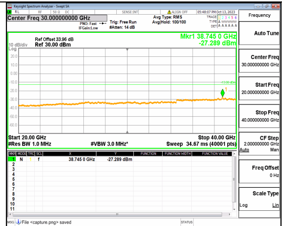
5A_n77(3700-3980MHz) (20GHz-40GHz) 80M DFT-s-OFDM QPSK Edge_1RB_Right Mid
