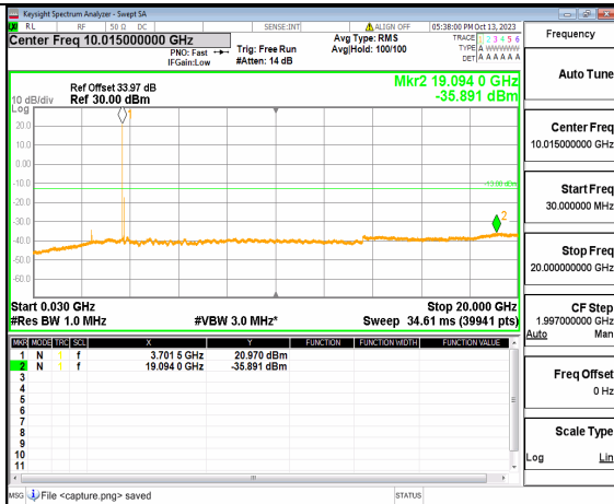
5A_n77(3700-3980MHz) (30MHz-20GHz) 80M DFT-s-OFDM QPSK Edge_1RB_Left Low
