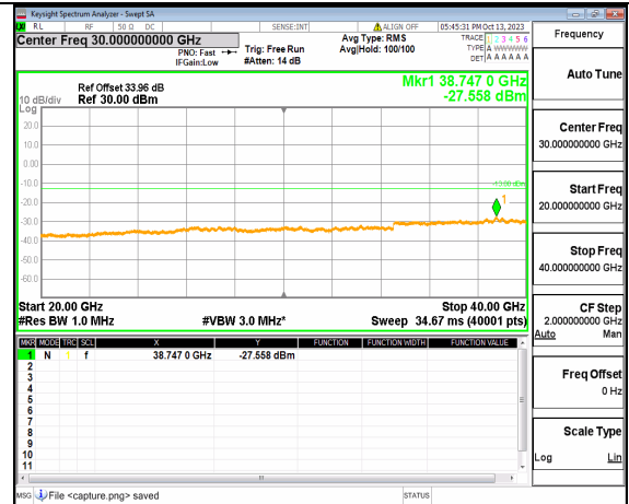
5A_n77(3700-3980MHz) (20GHz-40GHz) 80M DFT-s-OFDM QPSK Outer_Full Mid
