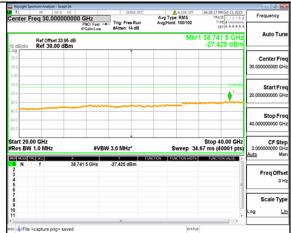
5A_n77(3700-3980MHz) (20GHz-40GHz) 90M DFT-s-OFDM QPSK Edge_1RB_Right High
