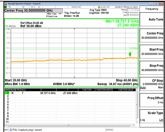
5A_n77(3700-3980MHz) (20GHz-40GHz) 90M DFT-s-OFDM BPSK Edge_1RB_Right Mid
