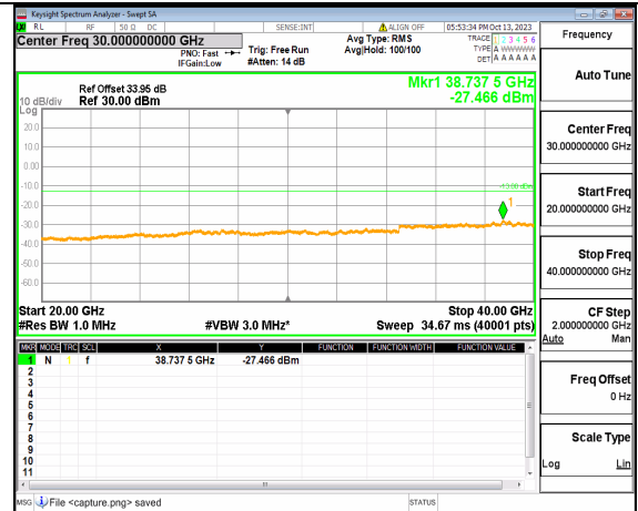
5A_n77(3700-3980MHz) (20GHz-40GHz) 80M DFT-s-OFDM QPSK Outer_Full High
