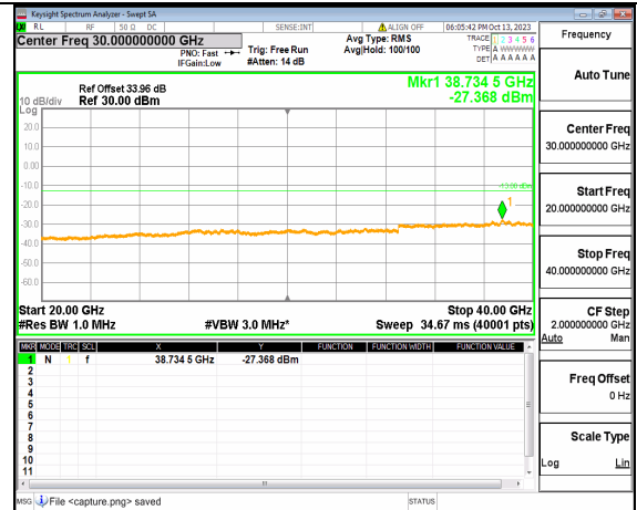
5A_n77(3700-3980MHz) (20GHz-40GHz) 90M DFT-s-OFDM BPSK Outer_Full Mid
