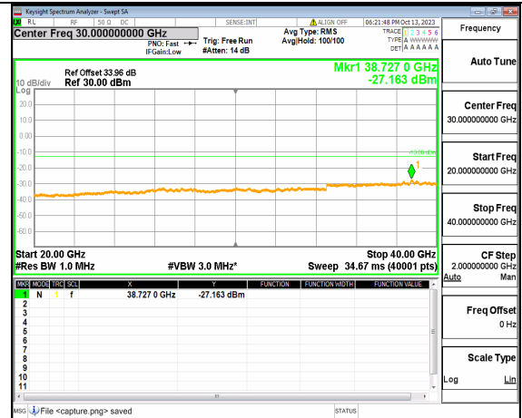
5A_n77(3700-3980MHz) (20GHz-40GHz) 100M DFT-s-OFDM BPSK Outer_Full Low
