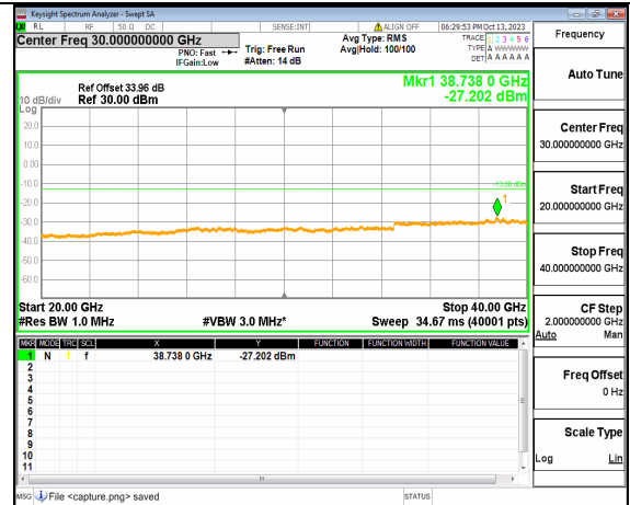
5A_n77(3700-3980MHz) (20GHz-40GHz) 100M DFT-s-OFDM BPSK Outer_Full Mid
