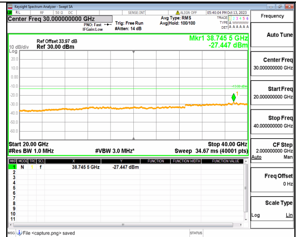
5A_n77(3700-3980MHz) (20GHz-40GHz) 80M DFT-s-OFDM QPSK Edge_1RB_Right Low
