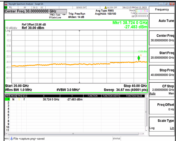
5A_n77(3700-3980MHz) (20GHz-40GHz) 90M DFT-s-OFDM QPSK Edge_1RB_Right Mid
