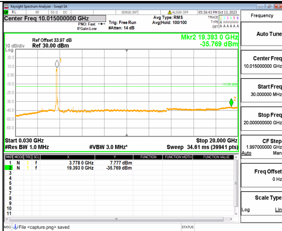
5A_n77(3700-3980MHz) (30MHz-20GHz) 80M DFT-s-OFDM QPSK Outer_Full Low
