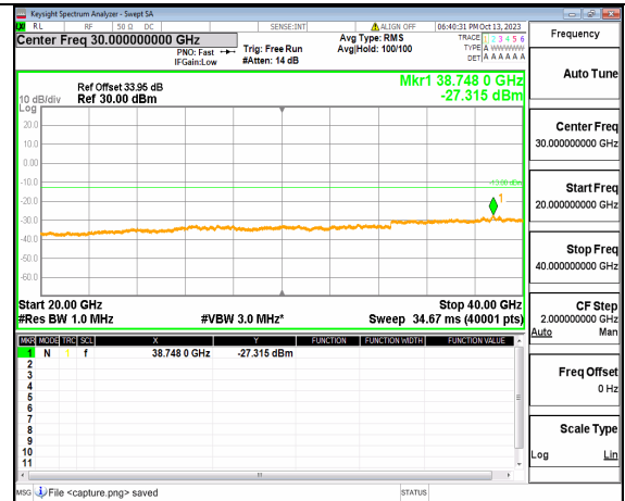
5A_n77(3700-3980MHz) (20GHz-40GHz) 100M DFT-s-OFDM BPSK Edge_1RB_Right High
