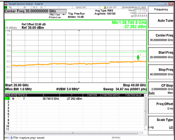
5A_n77(3700-3980MHz) (20GHz-40GHz) 80M DFT-s-OFDM BPSK Edge_1RB_Right Mid
