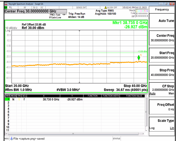
5A_n77(3700-3980MHz) (20GHz-40GHz) 60M DFT-s-OFDM BPSK Edge_1RB_Left High
