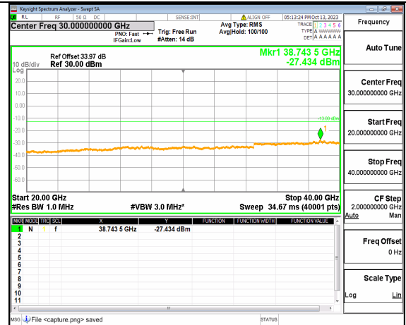
5A_n77(3700-3980MHz) (20GHz-40GHz) 70M DFT-s-OFDM QPSK Outer_Full Low
