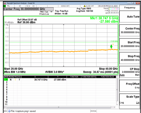
5A_n77(3700-3980MHz) (20GHz-40GHz) 70M DFT-s-OFDM QPSK Edge_1RB_Right Low
