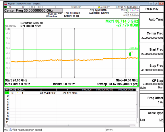
5A_n77(3700-3980MHz) (20GHz-40GHz) 60M DFT-s-OFDM QPSK Outer_Full Mid
