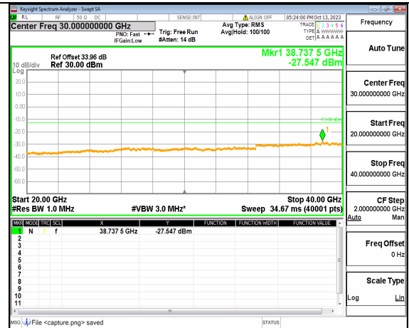
5A_n77(3700-3980MHz) (20GHz-40GHz) 70M DFT-s-OFDM QPSK Edge_1RB_Right Mid
