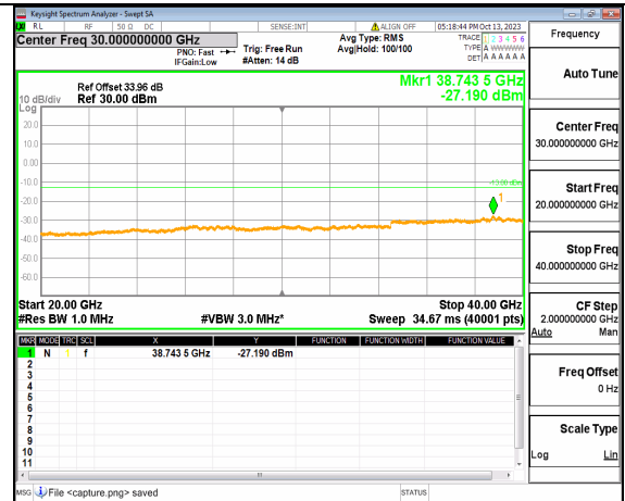
5A_n77(3700-3980MHz) (20GHz-40GHz) 70M DFT-s-OFDM BPSK Edge_1RB_Left Mid
