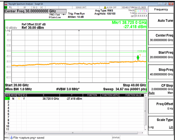
5A_n77(3700-3980MHz) (20GHz-40GHz) 30M DFT-s-OFDM QPSK Edge_1RB_Right Low
