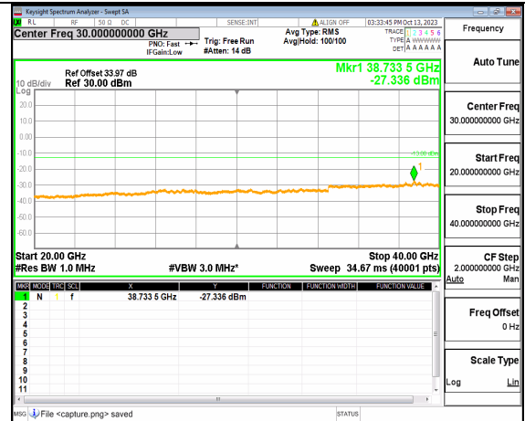
5A_n77(3700-3980MHz) (20GHz-40GHz) 30M DFT-s-OFDM BPSK Outer_Full Low
