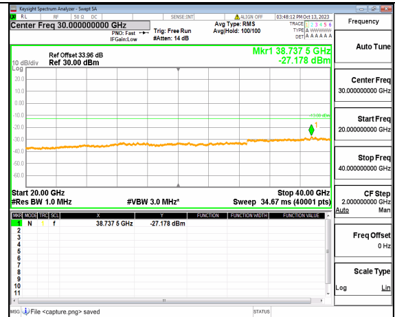
5A_n77(3700-3980MHz) (20GHz-40GHz) 30M DFT-s-OFDM QPSK Edge_1RB_Right Mid
