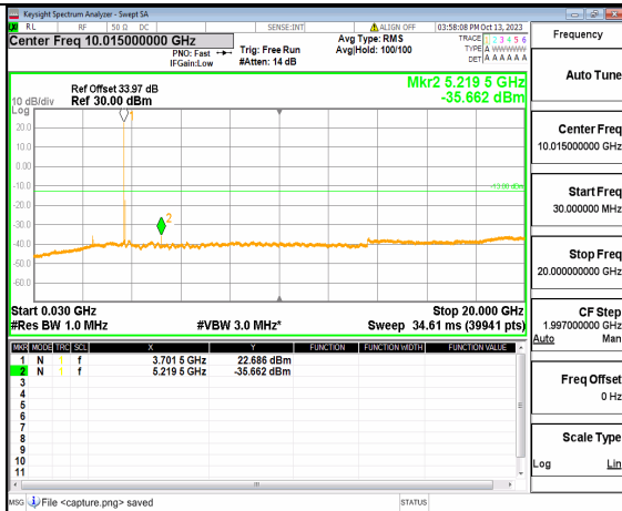
5A_n77(3700-3980MHz) (30MHz-20GHz) 40M DFT-s-OFDM BPSK Edge_1RB_Left Low
