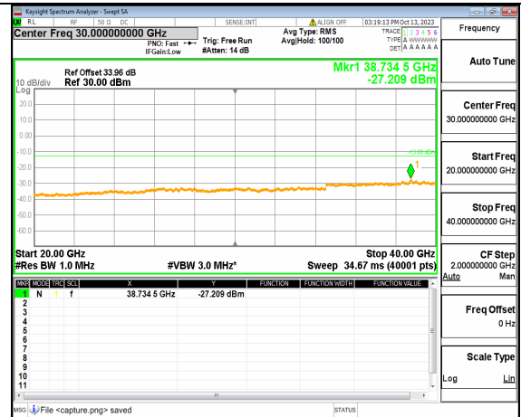
5A_n77(3700-3980MHz) (20GHz-40GHz) 20M DFT-s-OFDM BPSK Edge_1RB_Left Mid
