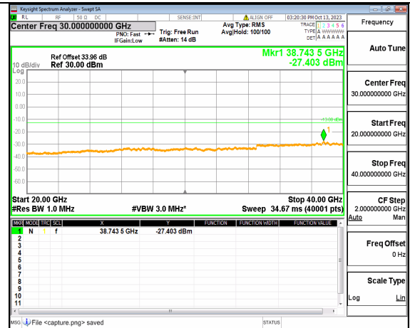
5A_n77(3700-3980MHz) (20GHz-40GHz) 20M DFT-s-OFDM BPSK Edge_1RB_Right Mid
