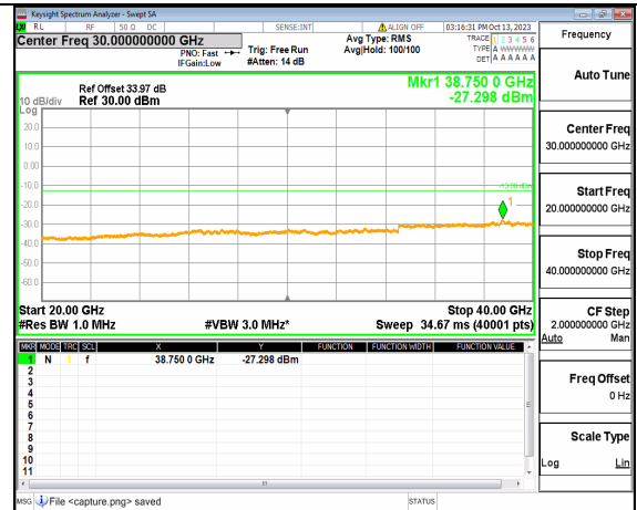
5A_n77(3700-3980MHz) (20GHz-40GHz) 20M DFT-s-OFDM QPSK Edge_1RB_Right Low
