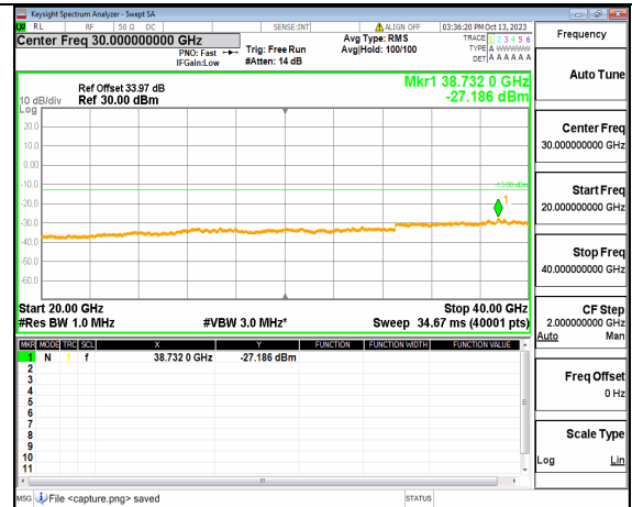
5A_n77(3700-3980MHz) (20GHz-40GHz) 30M DFT-s-OFDM BPSK Edge_1RB_Right Low
