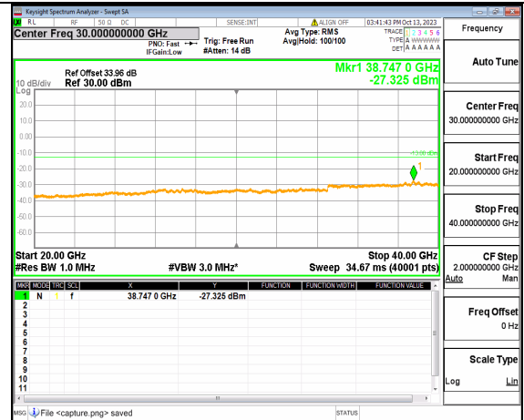
5A_n77(3700-3980MHz) (20GHz-40GHz) 30M DFT-s-OFDM BPSK Outer_Full Mid
