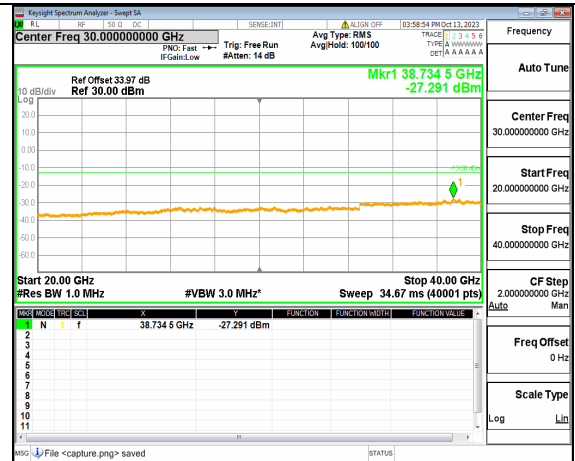
5A_n77(3700-3980MHz) (20GHz-40GHz) 40M DFT-s-OFDM BPSK Edge_1RB_Left Low
