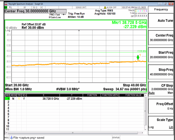
5A_n77(3700-3980MHz) (20GHz-40GHz) 30M DFT-s-OFDM QPSK Outer_Full Low
