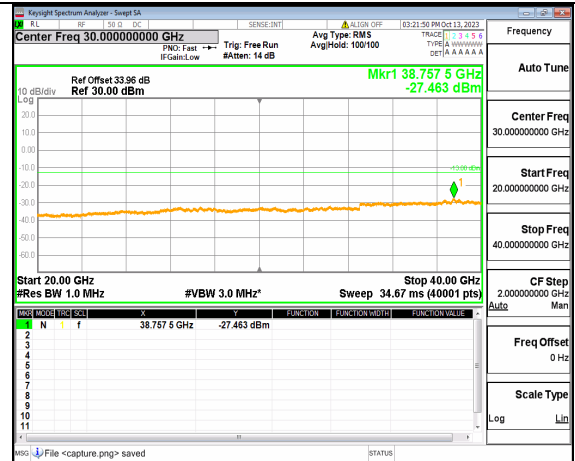
5A_n77(3700-3980MHz) (20GHz-40GHz) 20M DFT-s-OFDM QPSK Outer_Full Mid
