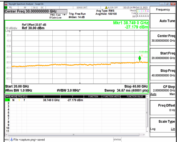
5A_n77(3700-3980MHz) (20GHz-40GHz) 20M DFT-s-OFDM QPSK Edge_1RB_Left Low
