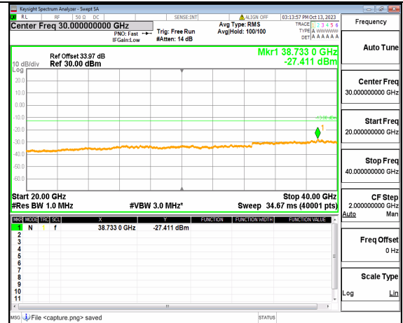
5A_n77(3700-3980MHz) (20GHz-40GHz) 20M DFT-s-OFDM QPSK Outer_Full Low
