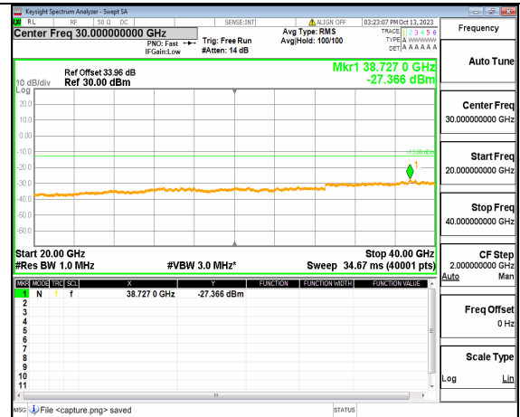
5A_n77(3700-3980MHz) (20GHz-40GHz) 20M DFT-s-OFDM QPSK Edge_1RB_Left Mid
