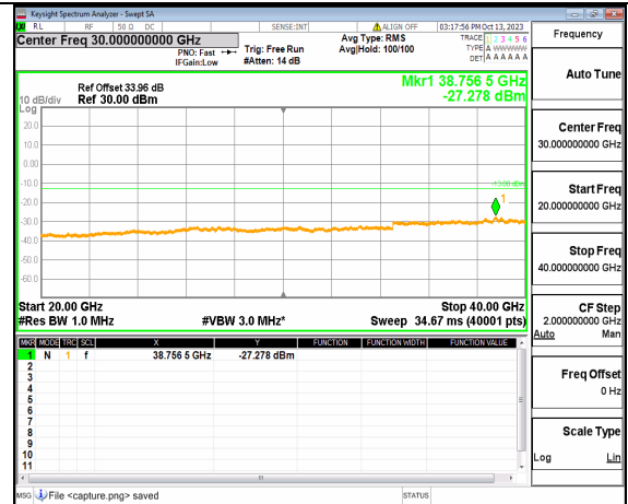
5A_n77(3700-3980MHz) (20GHz-40GHz) 20M DFT-s-OFDM BPSK Outer_Full Mid
