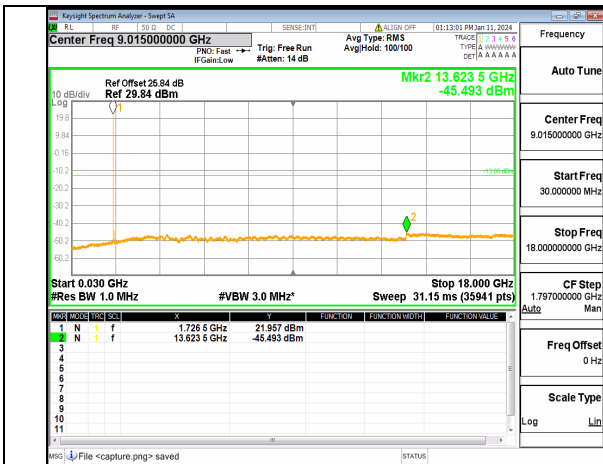
13A_n66 (30MHz-18GHz) 40M DFT-s-OFDM QPSK Inner_1RB_Left Mid
