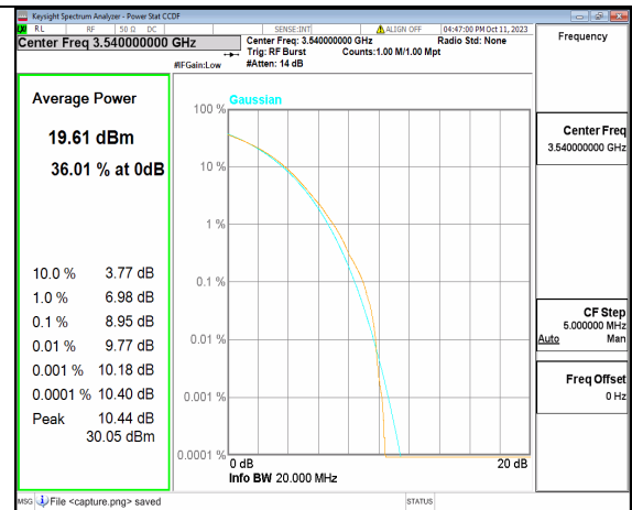
5A_n77(3450-3550MHz) 20M CP-OFDM 256QAM Outer_Full High
