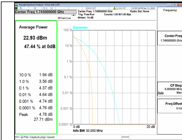
13A_n66 30M DFT-s-OFDM BPSK Outer_Full Mid
