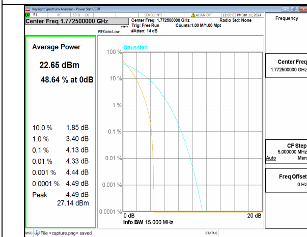
13A_n66 15M DFT-s-OFDM BPSK Outer_Full High
