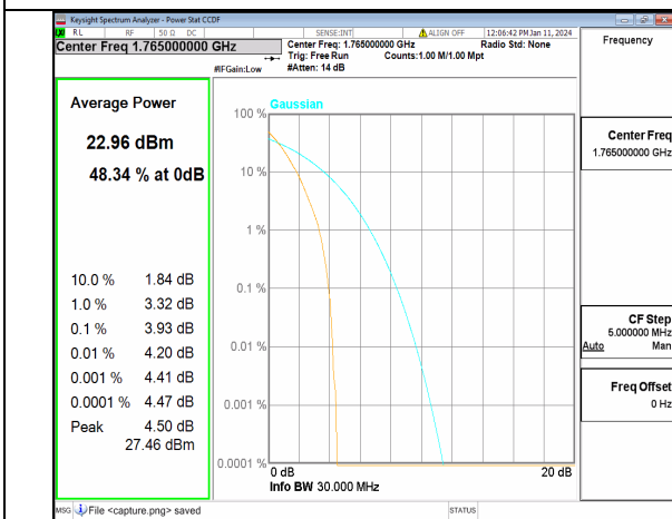
13A_n66 30M DFT-s-OFDM BPSK Outer_Full High
