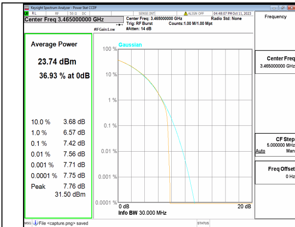
5A_n77(3450-3550MHz) 30M CP-OFDM QPSK Outer_Full Low
