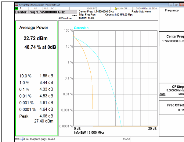
13A_n66 15M DFT-s-OFDM BPSK Outer_Full Mid
