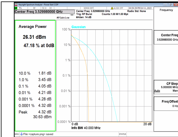
5A_n77(3450-3550MHz) 40M DFT-s-OFDM BPSK Outer_Full High
