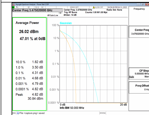
5A_n77(3450-3550MHz) 50M DFT-s-OFDM BPSK Outer_Full Low
