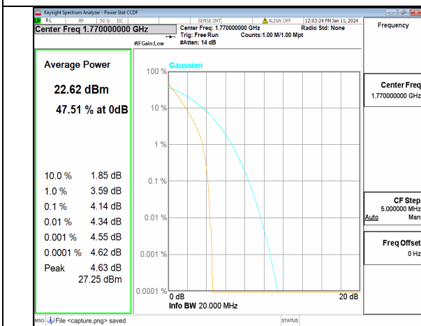
13A_n66 20M DFT-s-OFDM BPSK Outer_Full High
