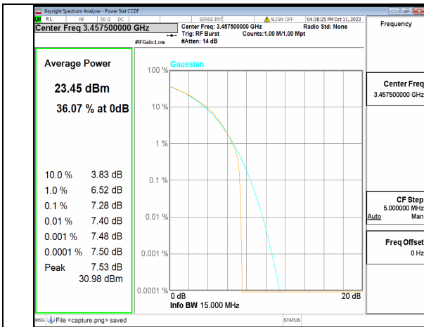
5A_n77(3450-3550MHz) 15M CP-OFDM QPSK Outer_Full Low
