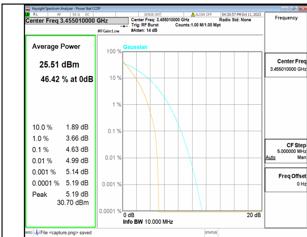
5A_n77(3450-3550MHz) 10M DFT-s-OFDM BPSK Outer_Full Low
