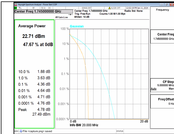
13A_n66 20M DFT-s-OFDM BPSK Outer_Full Mid
