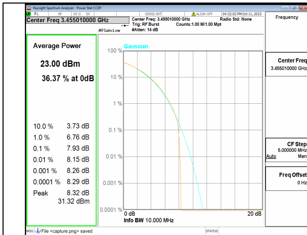
5A_n77(3450-3550MHz) 10M CP-OFDM QPSK Outer_Full Low
