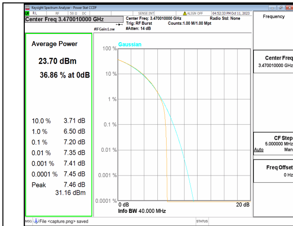
5A_n77(3450-3550MHz) 40M CP-OFDM QPSK Outer_Full Low
