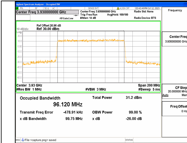
5A_n77(3700-3980MHz) 100M DFT-s-OFDM 256QAM Outer_Full High
