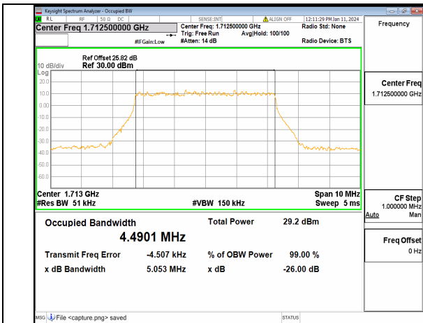
13A_n66 5M DFT-s-OFDM 16QAM Outer_Full Low
