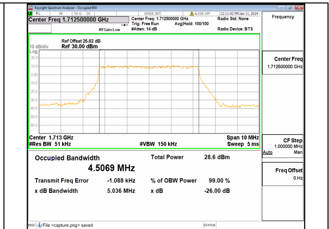
13A_n66 5M DFT-s-OFDM 64QAM Outer_Full Low
