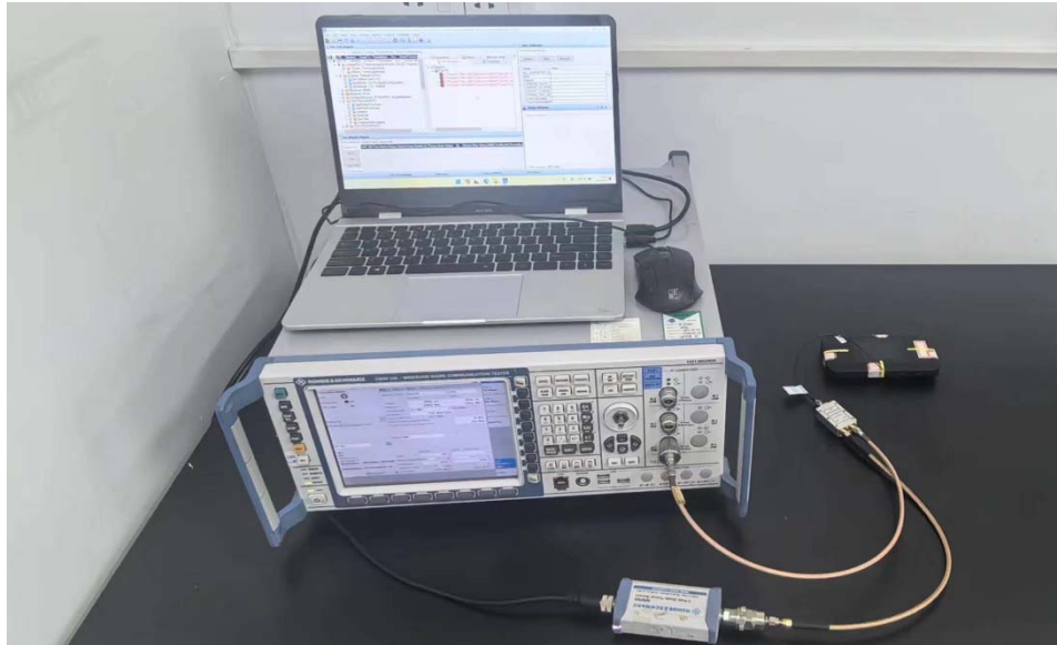
Test setup
