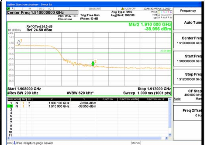
B2 / 20MHz / High CH / QPSK / FULL RB
