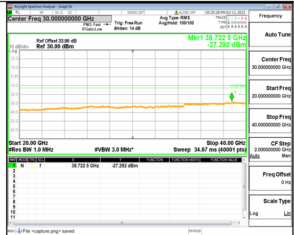
5A_n77(3700-3980MHz) (20GHz-40GHz) 70M DFT-s-OFDM BPSK Outer_Full High
