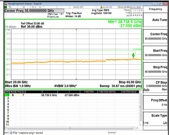
5A_n77(3700-3980MHz) (20GHz-40GHz) 70M DFT-s-OFDM QPSK Outer_Full Mid
