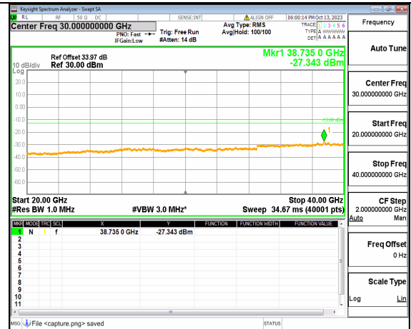
5A_n77(3700-3980MHz) (20GHz-40GHz) 90M DFT-s-OFDM BPSK Edge_1RB_Right Low
