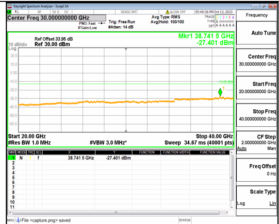
5A_n77(3700-3980MHz) (20GHz-40GHz) 80M DFT-s-OFDM BPSK Outer_Full High
