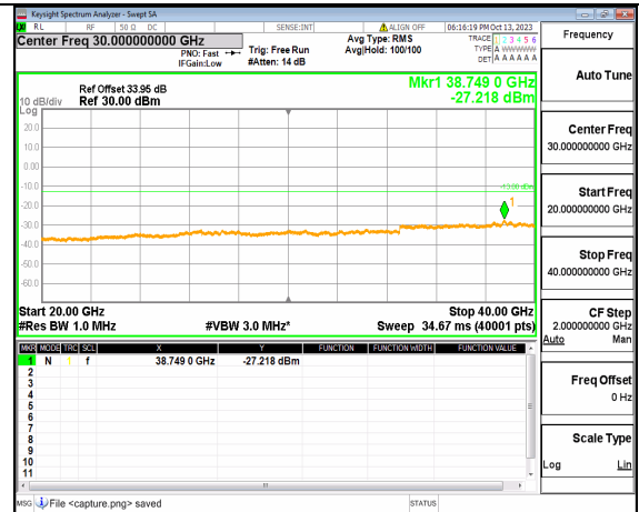
5A_n77(3700-3980MHz) (20GHz-40GHz) 90M DFT-s-OFDM BPSK Edge_1RB_Right High
