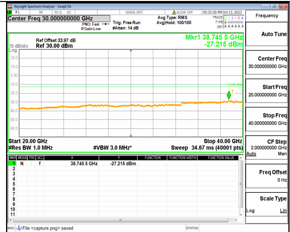
5A_n77(3700-3980MHz) (20GHz-40GHz) 80M DFT-s-OFDM BPSK Outer_Full Low
