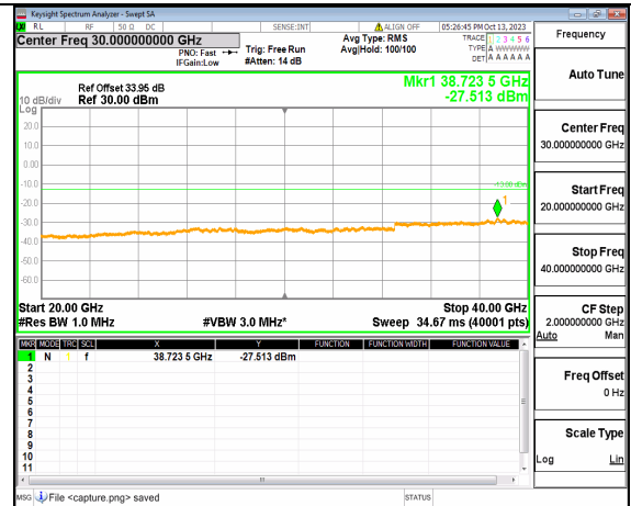
5A_n77(3700-3980MHz) (20GHz-40GHz) 70M DFT-s-OFDM BPSK Edge_1RB_Left High
