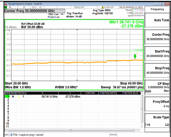
5A_n77(3700-3980MHz) (20GHz-40GHz) 100M DFT-s-OFDM BPSK Edge_1RB_Right Mid
