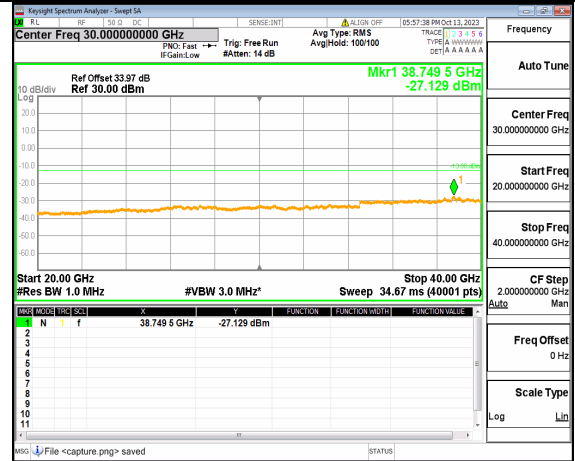
5A_n77(3700-3980MHz) (20GHz-40GHz) 90M DFT-s-OFDM BPSK Outer_Full Low
