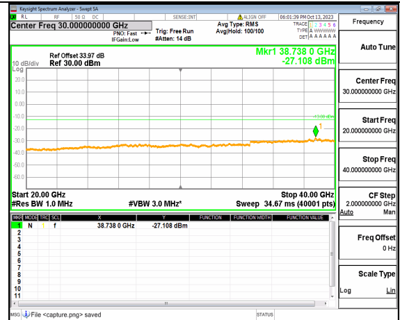
5A_n77(3700-3980MHz) (20GHz-40GHz) 90M DFT-s-OFDM QPSK Outer_Full Low
