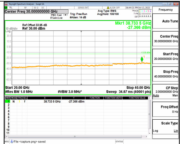
5A_n77(3700-3980MHz) (20GHz-40GHz) 100M DFT-s-OFDM QPSK Edge_1RB_Right High
