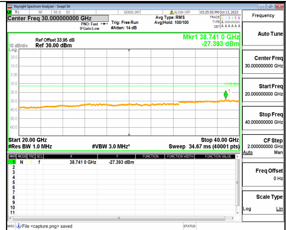
5A_n77(3700-3980MHz) (20GHz-40GHz) 20M DFT-s-OFDM BPSK Outer_Full High
