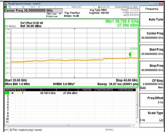
5A_n77(3700-3980MHz) (20GHz-40GHz) 20M DFT-s-OFDM QPSK Edge_1RB_Right Mid
