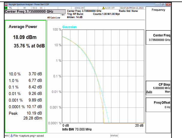
5A_n77(3700-3980MHz) 70M CP-OFDM 256QAM Outer_Full Low
