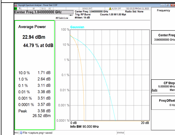
5A_n77(3700-3980MHz) 90M DFT-s-OFDM BPSK Outer_Full Mid
