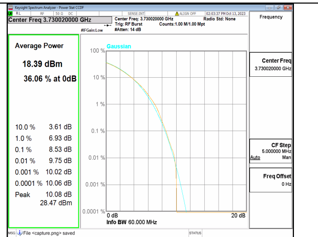
5A_n77(3700-3980MHz) 60M CP-OFDM 256QAM Outer_Full Low
