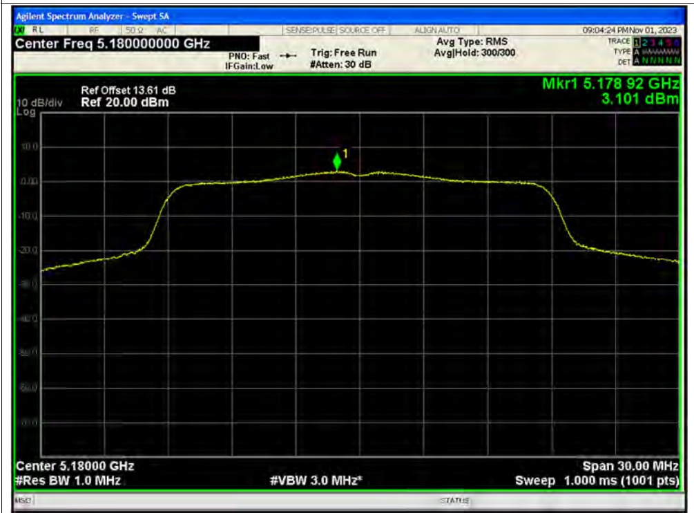
PSD NVNT ac20 5180MHz Ant2 MIMO
