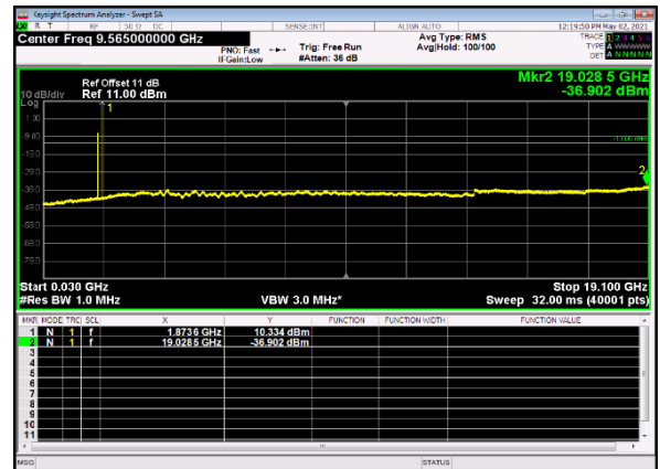
B66_n2(15M)_DFT-s-OFDM_QPSK_Edge_ 1RB_Left_Mid_CH
