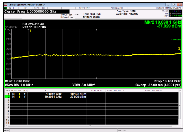
B66_n2(10M)_DFT-s-OFDM_QPSK_Edge_1RB_Left_High_CH
