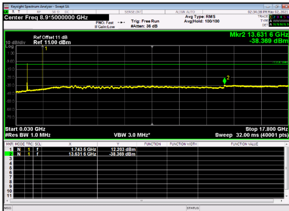
B13_n66(5M)_DFT-s-OFDM_BPSK_Edge_ 1RB_Left_Mid_CH
