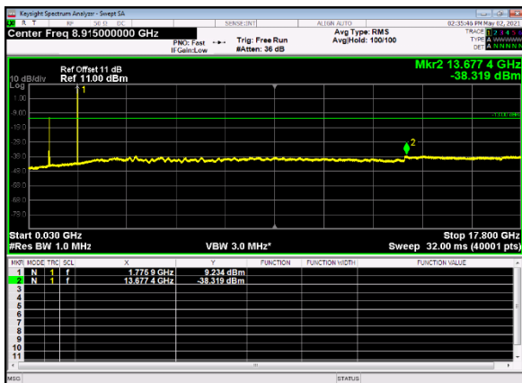
B13_n66(5M)_DFT-s-OFDM_BPSK_Edge_ 1RB_Left_High_CH
