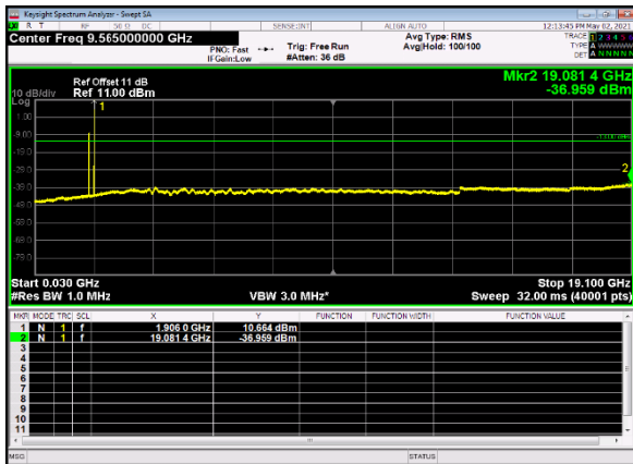
B66_n2(5M)_DFT-s-OFDM_BPSK_Edge_ 1RB_Left_High_CH
