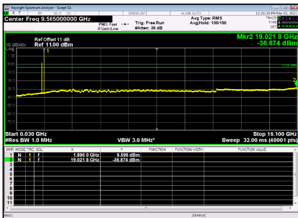
B66_n2(15M)_DFT-s-OFDM_BPSK_Edge_ 1RB_Left_High_CH
