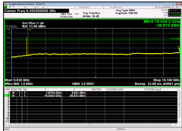
B66_n2(10M)_DFT-s-OFDM_QPSK_Edge_1RB_Left_Mid_CH
