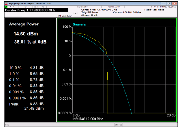
B13_n66(10M)_DFT-s-OFDM_PI_2-BPSK_Edge _1RB_Left_High_CH
