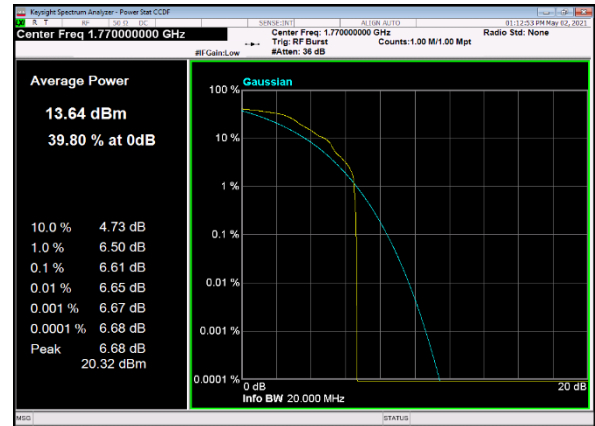
B13_n66(20M)_DFT-s-OFDM_PI_2-BPSK_Edge _1RB_Left_High_CH
