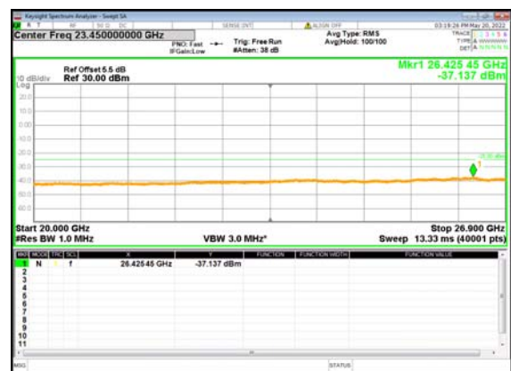
B66_n41(60M)_DFT-s-OFDM_BPSK_Edge_1R B_Left_Mid_CH
