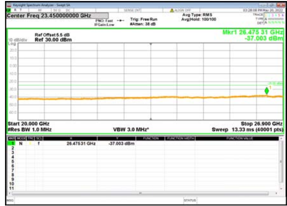
B66_n41(100M)_DFT-s-OFDM_QPSK_Edge_1 RB_Left_Mid_CH
