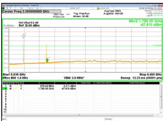
B66_n71(20M)_DFT-s-OFDM_BPSK_Edge_1R B_Left_High_CH
