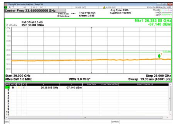
B66_n41(40M)_DFT-s-OFDM_BPSK_Edge_1R B_Left_High_CH
