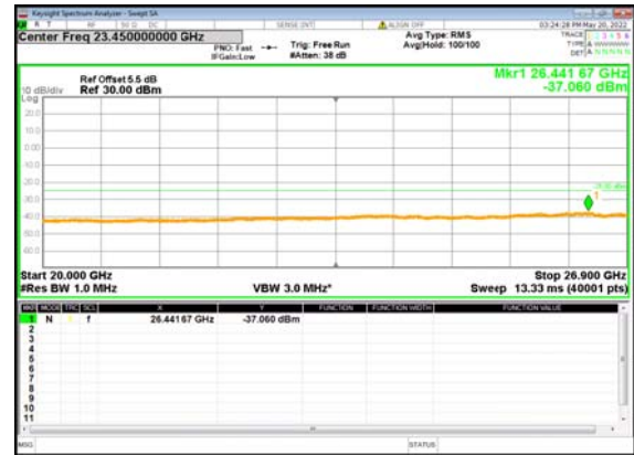
B66_n41(100M)_DFT-s-OFDM_BPSK_Edge_1 RB_Left_Low_CH
