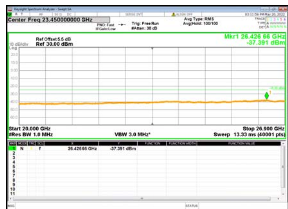
B66_n41(40M)_DFT-s-OFDM_BPSK_Edge_1R B_Left_Mid_CH
