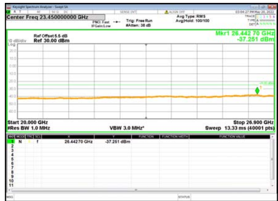
B66_n41(20M)_DFT-s-OFDM_BPSK_Edge_1R B_Left_Mid_CH
