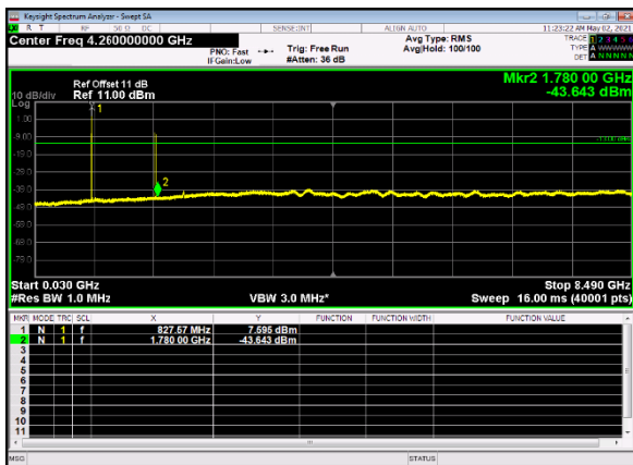
B66_n5(20M)_DFT-s-OFDM_BPSK_Edge_1RB_Left_Mid_CH
