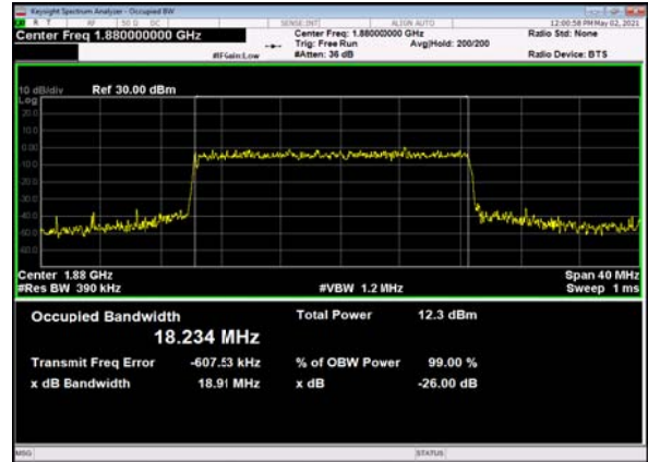
B66_n2(20M)_DFT-s-OFDM_QPSK_Outer_Full_Mid_CH
