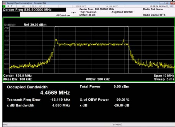
B66_n5(5M)_DFT-s-OFDM_PI_2-BPSK_Outer_Full_Mid_CH
