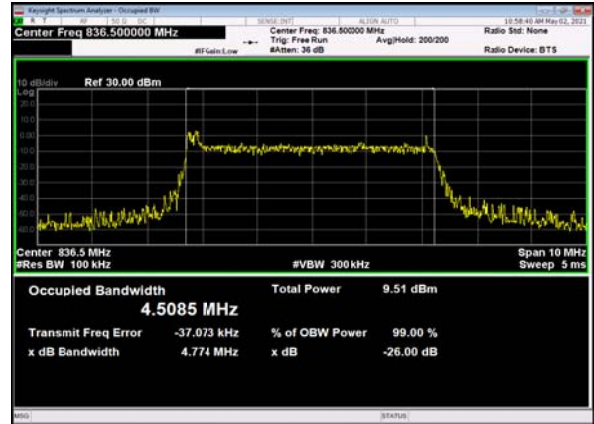
B66_n5(5M)_DFT-s-OFDM_QPSK_Outer_Full_Mid_CH
