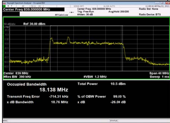
B66_n5(20M)_DFT-s-OFDM_PI_2-BPSK_Outer_Full_High_CH
