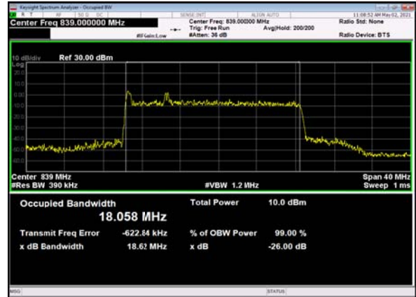
B66_n5(20M)_DFT-s-OFDM_QPSK_Outer_Full_High_CH
