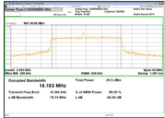
B66_n41(20M)_CP-OFDM_QPSK_Outer_Fu ll_Mid_CH
