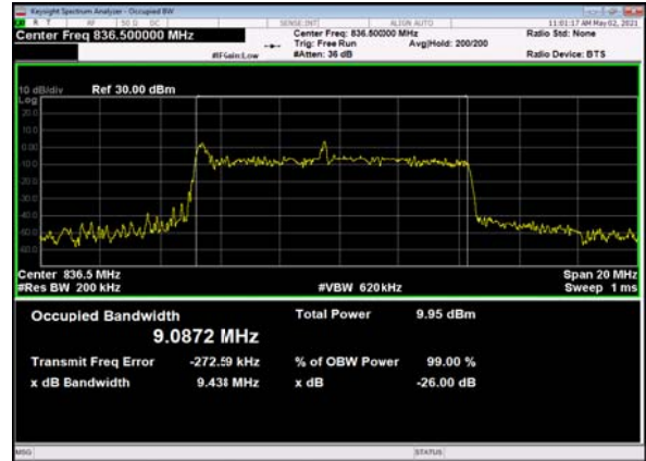
B66_n5(10M)_DFT-s-OFDM_QPSK_Outer_Full_Mid_CH
