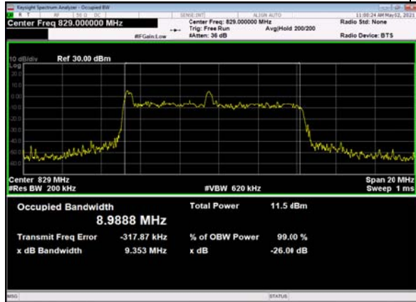
B66_n5(10M)_DFT-s-OFDM_PI_2-BPSK_Outer_Full_Low_CH
