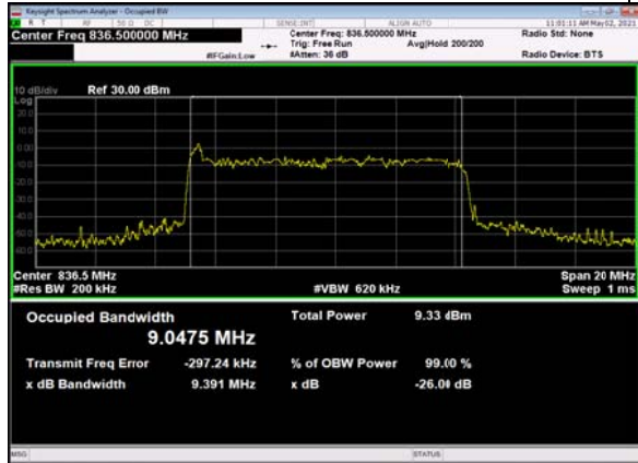
B66_n5(10M)_DFT-s-OFDM_PI_2-BPSK_Outer_Full_Mid_CH
