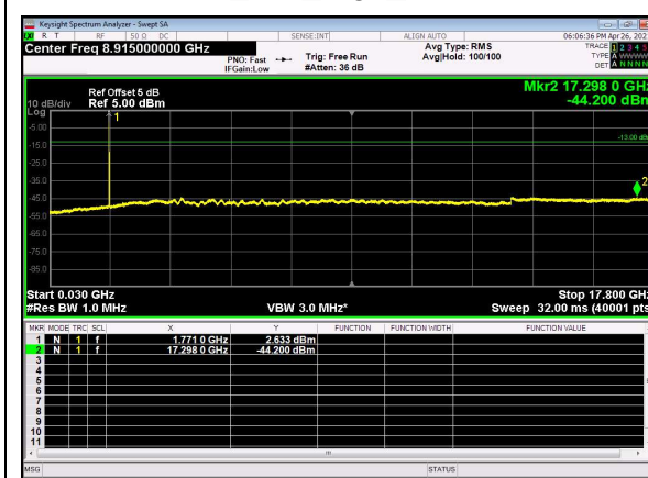
N66(10M)_DFT-s-OFDM_BPSK_Edge_1R B_Left_High_CH
