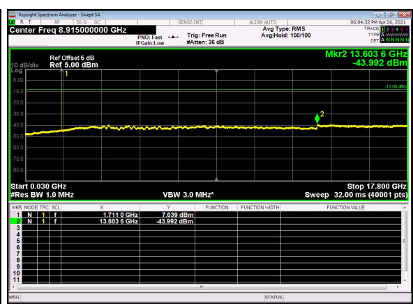
N66(10M)_DFT-s-OFDM_QPSK_Edge_1R B_Left_Low_CH
