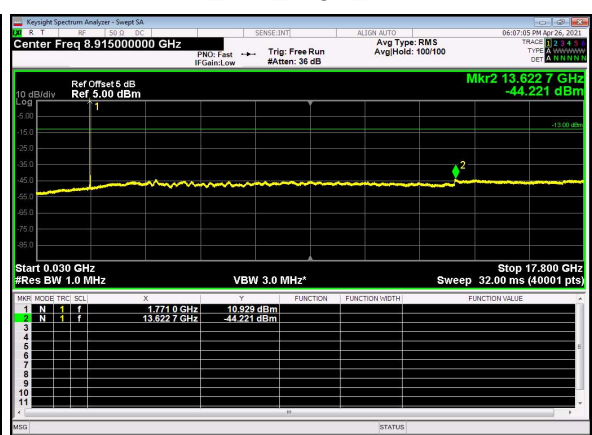
N66(10M)_DFT-s-OFDM_QPSK_Edge_1R B_Left_High_CH
