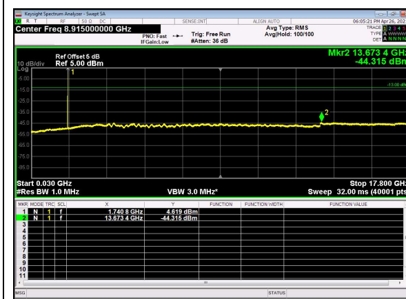
N66(10M)_DFT-s-OFDM_BPSK_Edge_1R B_Left_Mid_CH
