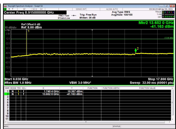
N66(10M)_DFT-s-OFDM_QPSK_Edge_1R B_Left_Mid_CH
