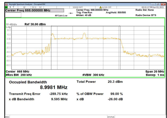
N71(10M)_CP-OFDM_QPSK_Outer_Full_Lo w_CH
