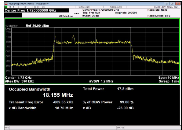
N66(20M)_DFT-s-OFDM_64 QAM_Outer_Full_Low_CH
