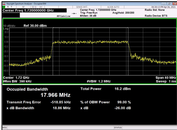
N66(20M)_DFT-s-OFDM_16 QAM_Outer_Full_Low_CH
