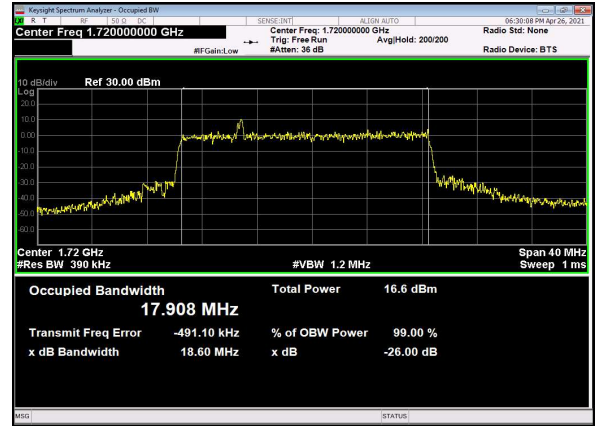
N66(20M)_DFT-s-OFDM_QPSK_Outer_Full Low_CH
