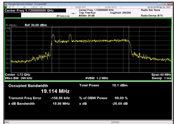
N66(20M)_CP-OFDM_QPSK_Outer_Full_Lo w_CH
