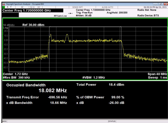
N66(20M)_DFT-s-OFDM_256 QAM_Outer_Full_Low_CH
