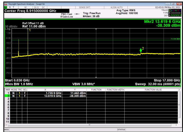
B13_N66(20M)_DFT-s-OFDM_QPSK_Edge_1RB_Left_Mid_CH
