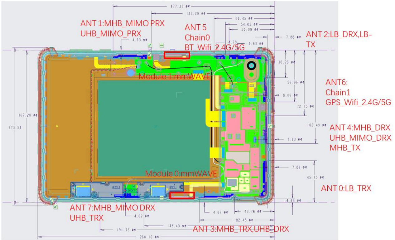
Fig.11.1 EUT Antenna Locations
