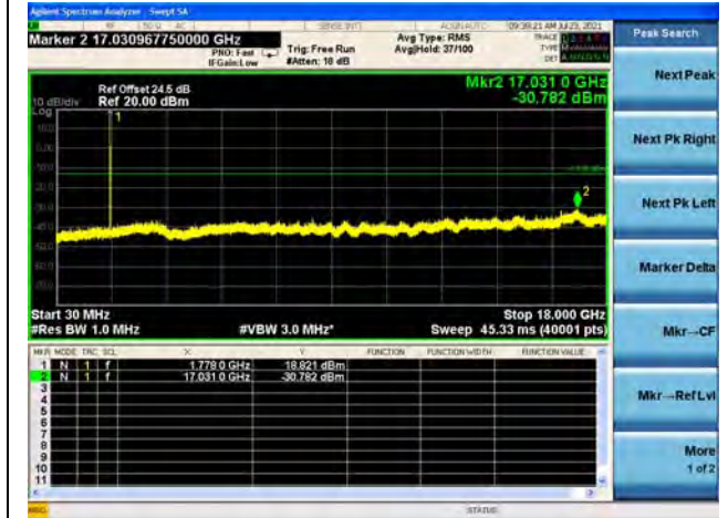
Band66 / 3MHz / High CH / 64QAM
