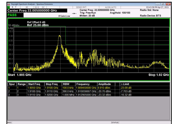
N2(20M)_DFT-s-OFDM_QPSK_Edge_1RB_Ri ght_High_CH
