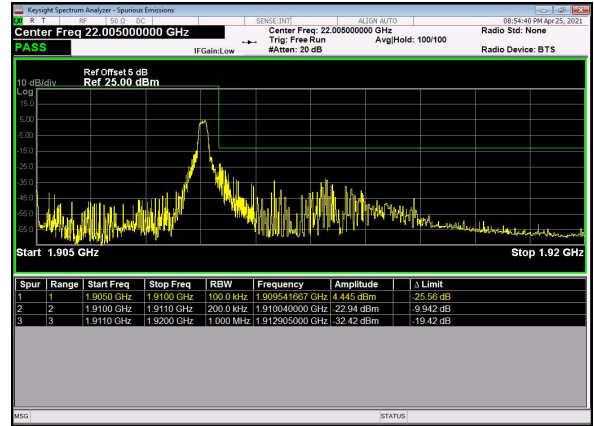
N2(10M)_DFT-s-OFDM_QPSK_Edge_1RB_Ri ght_High_CH
