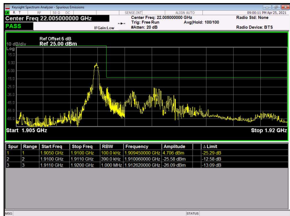
N2(20M)_DFT-s-OFDM_BPSK_Edge_1RB_Rig ht_High_CH
