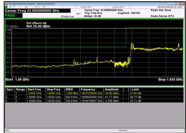
N2(20M)_DFT-s-OFDM_QPSK_Outer_Full_Lo w_CH
