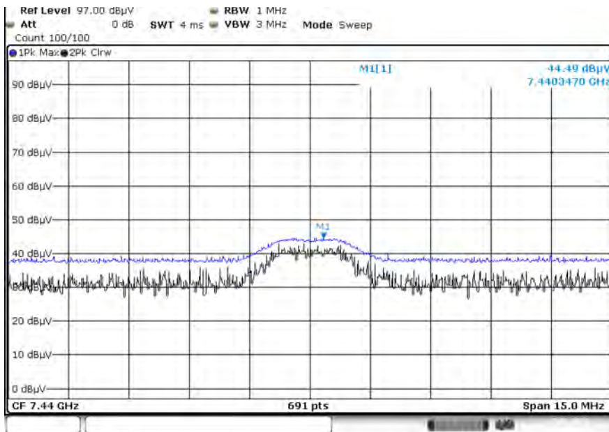
Radiated Spurious Emissions plot – Peak Reading ( \pi/4 DQPSK, Ch.78 3rd Harmonic, X-H)
