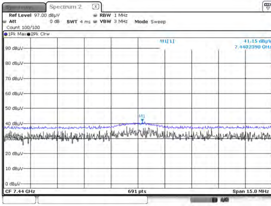
Radiated Spurious Emissions plot – Peak Reading (8DPSK, Ch.78 3rd Harmonic, X-H)
