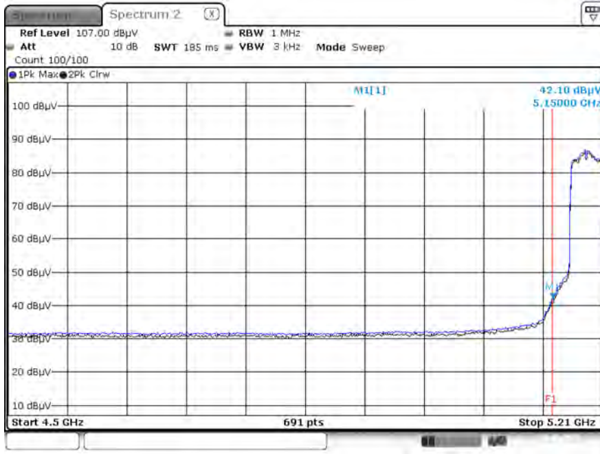
Average Reading (802.11ac(VHT40), Ch.38)
