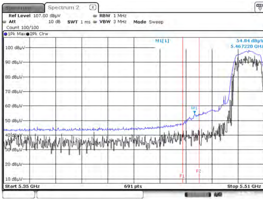
Peak Reading (802.11a, Ch.100)
