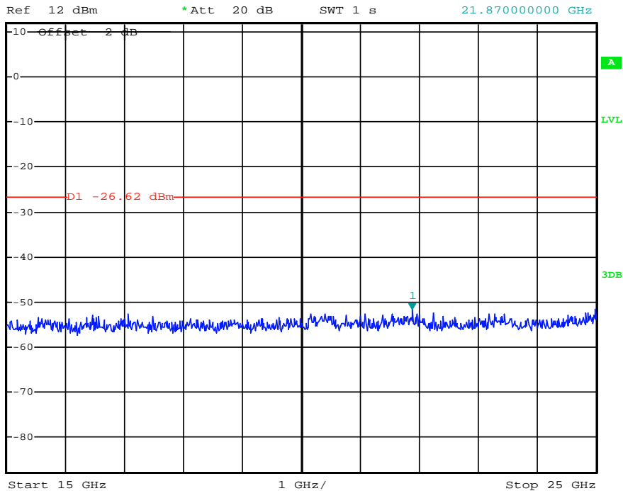
(Plot 4.7 B2: Channel 19: 2440MHz)
