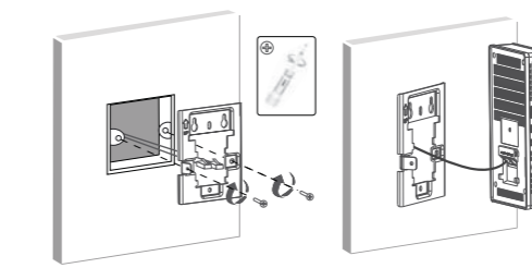
Fig 3-1 Install AP into Wall Socket
