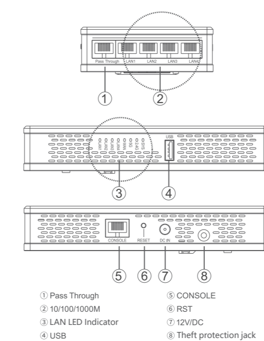
Fig A-4 Router/AP Port Diagram
