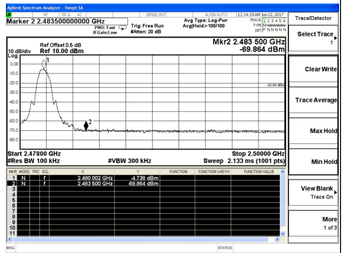
Channel 39 / 2480 MHz
