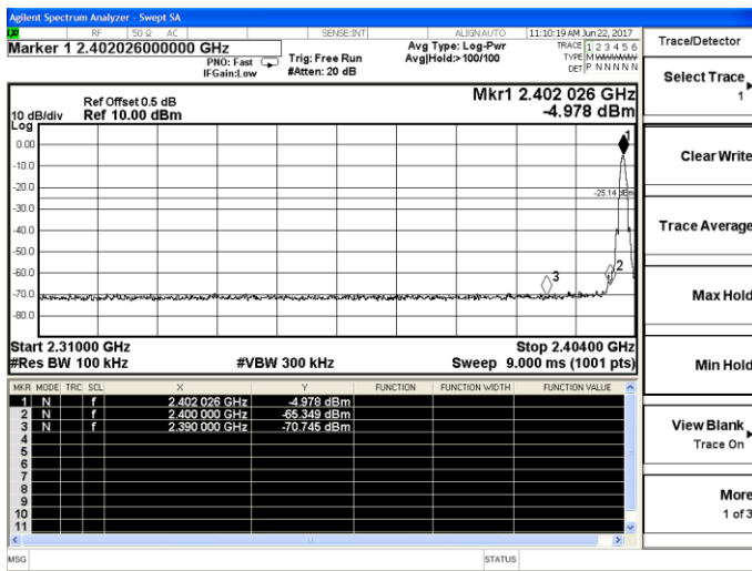
Channel 0 / 2402 MHz
