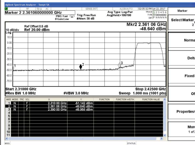
802.11n-HT20-Low channel(Peak)
