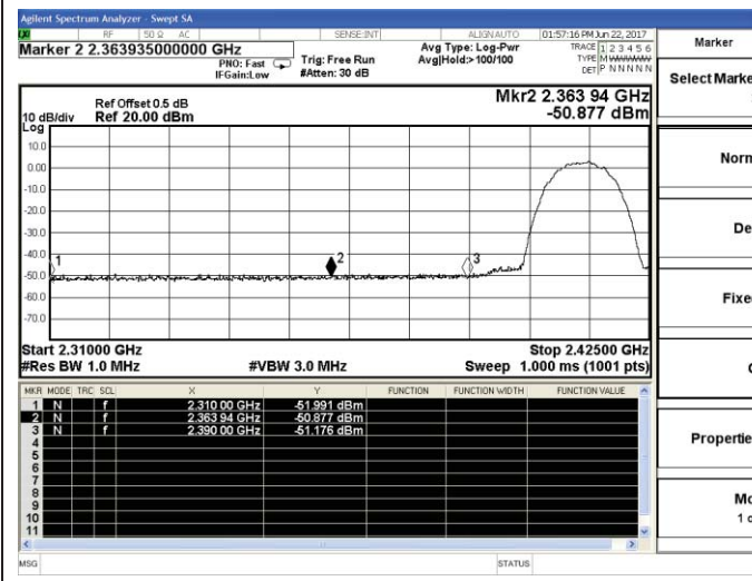
802.11b-Low channel(Peak)
