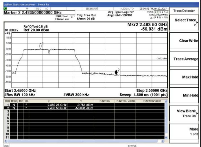
802.11g-High channel
