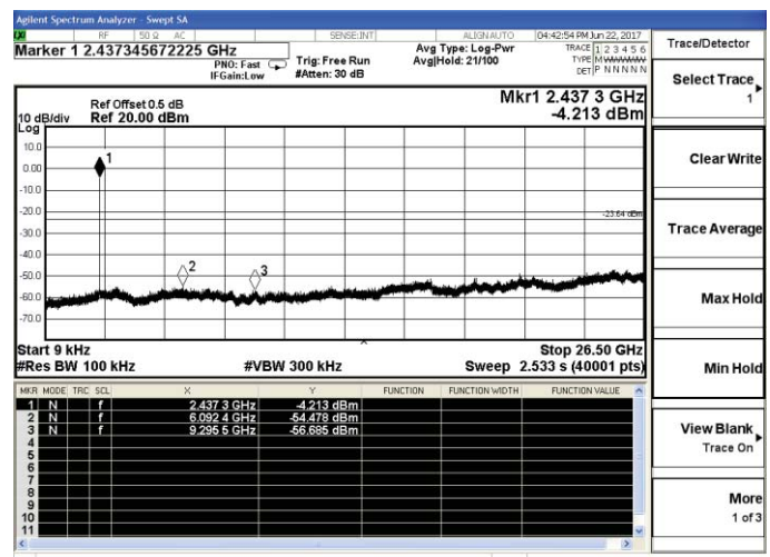
802.11b-Middle channel
