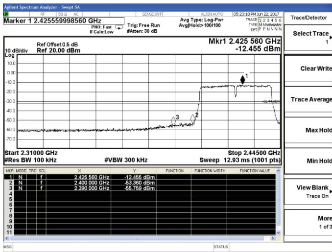
802.11n-HT40-Low channel
