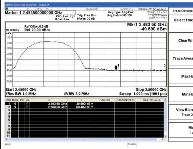
802.11b-High channel(Peak)
