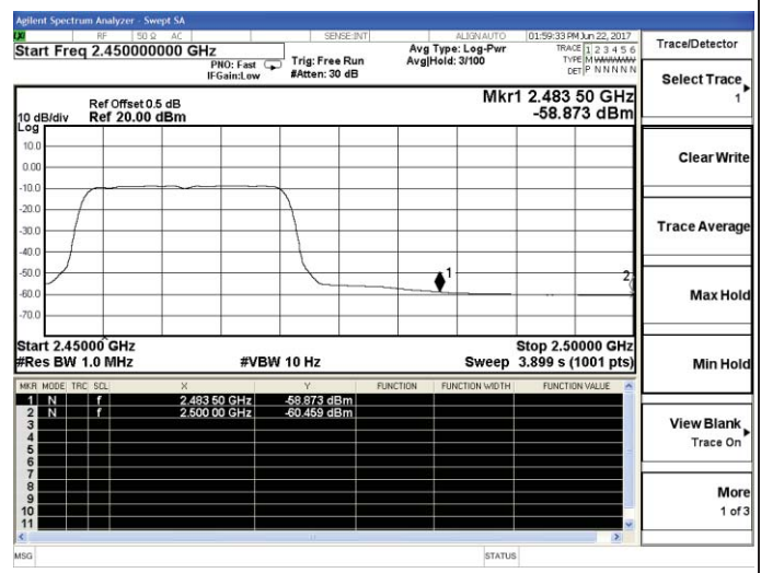
802.11g-High channel(Average)
