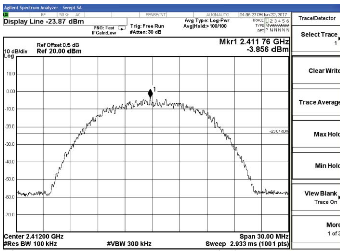
IEEE 802.11b-Channel 1 / 2412 MHz
