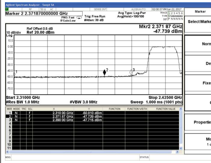
802.11g-Low channel(Peak)
