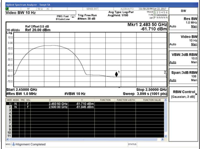
802.11b-High channel(Average)
