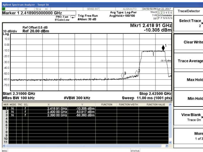
802.11g-Low channel
