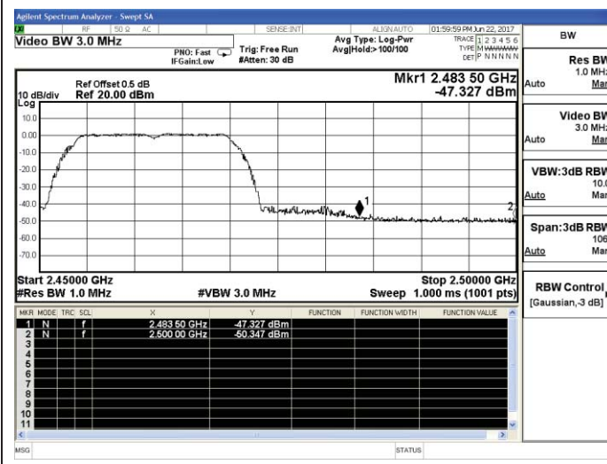
802.11g-High channel(Peak)
