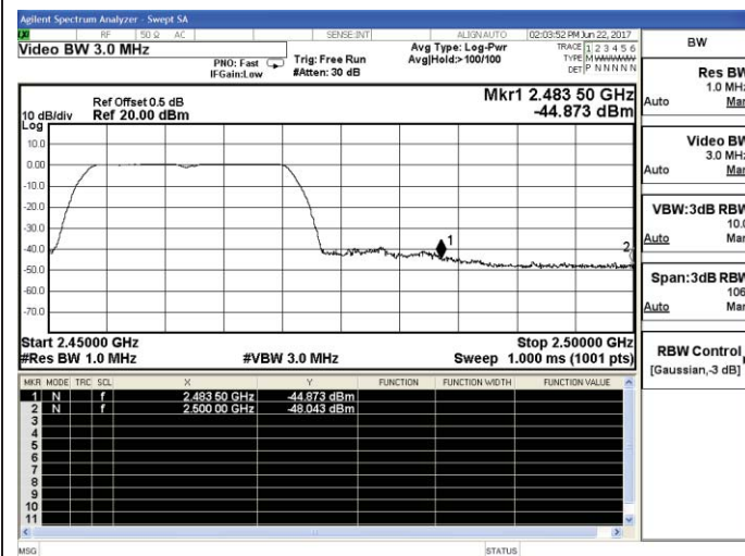
802.11n-HT20-High channel(Peak)
