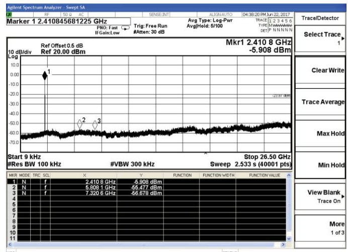
802.11b-Low channel
